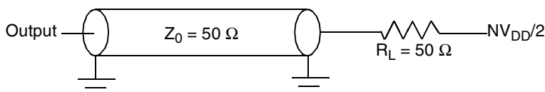
Figure 33. Timers AC Test Load
