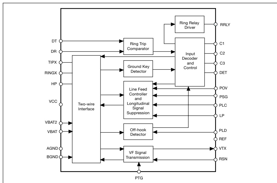
Figure 1. Block diagram.
