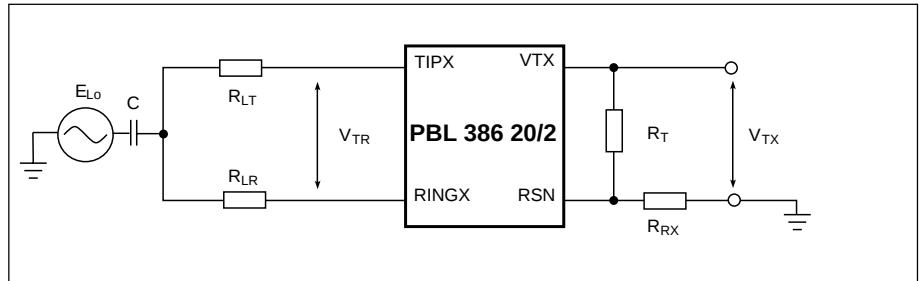
Figure 3. Longitudinal to metallic ( B_{\text{LME}} ) and Longitudinal to four-wire ( B_{\text{LFE}} ) balance
