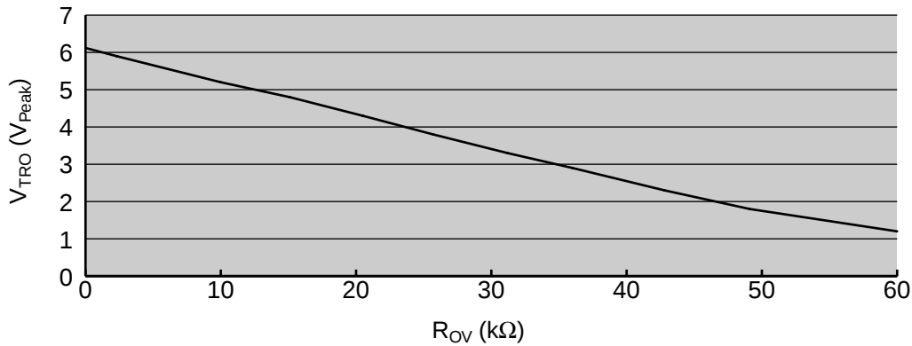
Figure 11. Programmable overhead voltage (POV). R_L = 600 \Omega or \infty .
