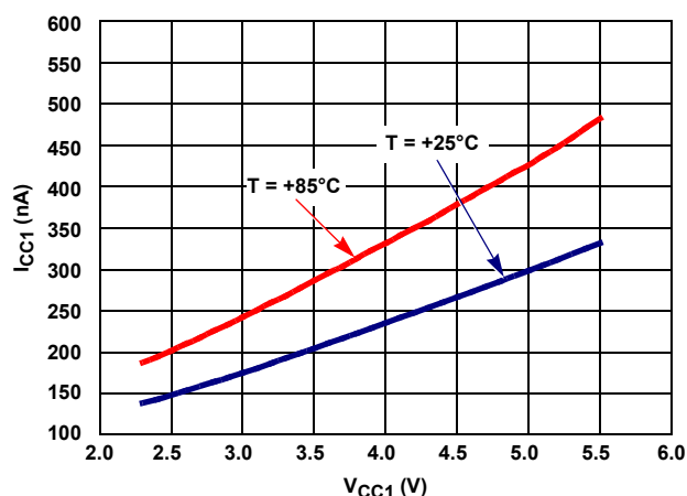
FIGURE 12. I_{CC1} DISABLED CURRENT vs V_{CC1} (ISL33001)
