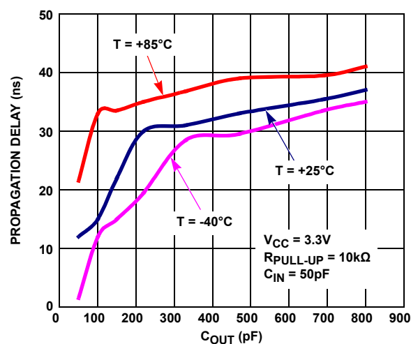
FIGURE 24. PROPAGATION DELAY H-L vs C_{OUT}
