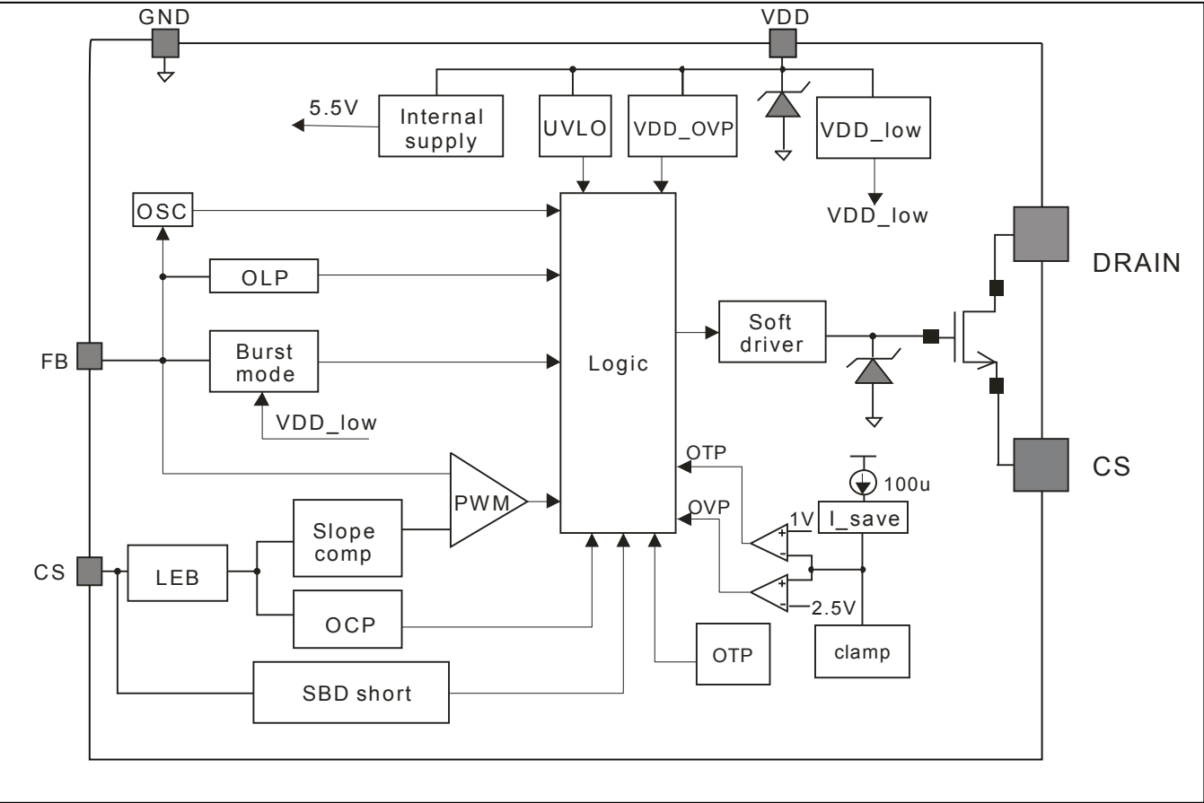
Internal Block Diagram
