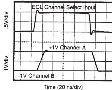
Large Signal Channel-to-Channel Switching
