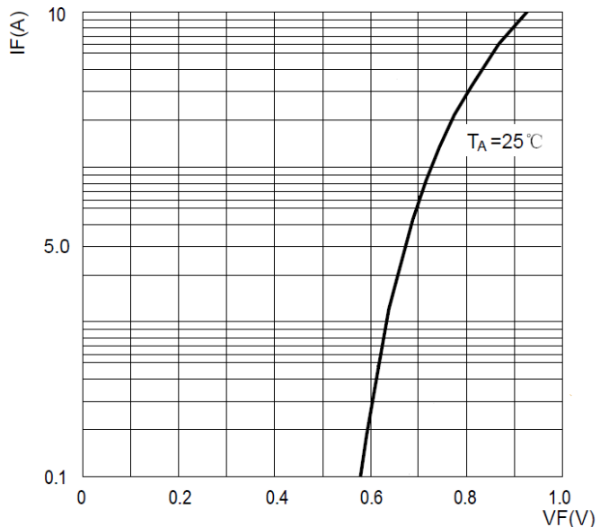
Fig2 : Instantaneous Forward Voltage
