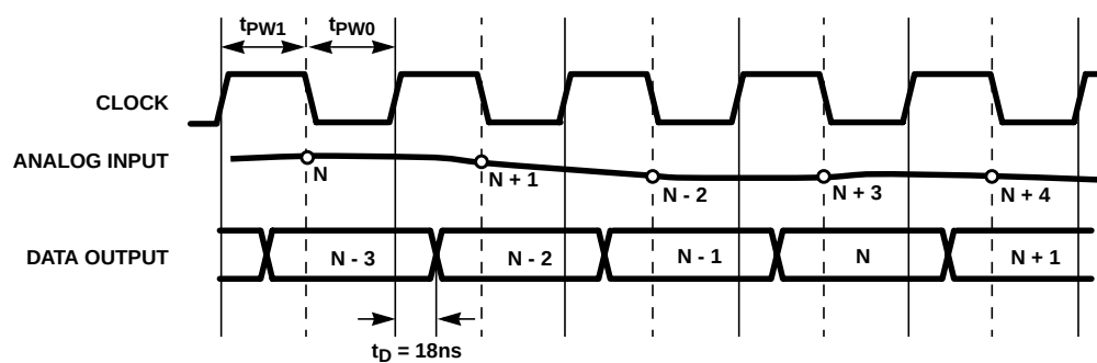
FIGURE 4. TIMING CHART 1
