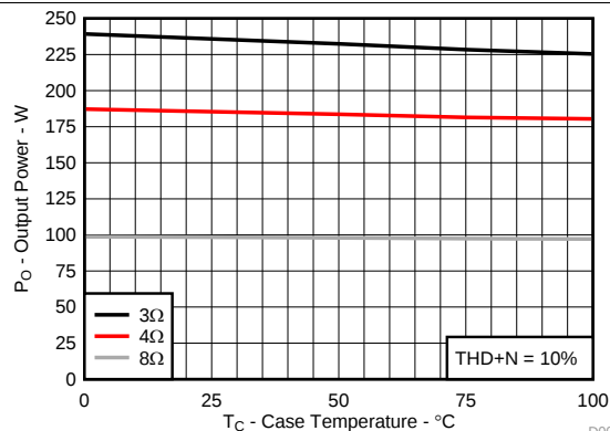
Figure 8. Output Power vs Case Temperature
