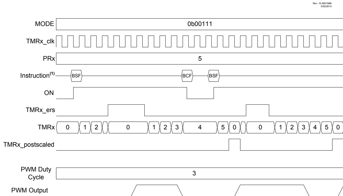
Figure 26-6. Level-Triggered Hardware Limit Mode Timing Diagram (MODE = 00111)
