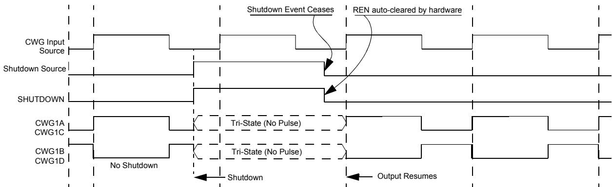
Figure 31-18. SHUTDOWN FUNCTIONALITY, AUTO-RESTART ENABLED (REN = 1, LSAC = 01, LSBD = 01)
