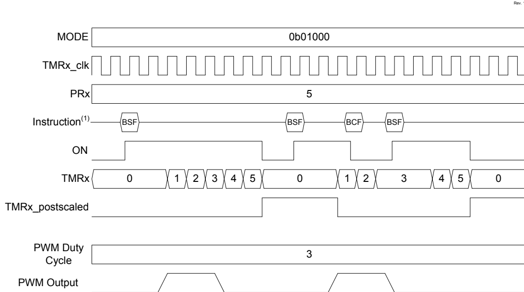
Figure 26-7. Software Start One-shot Mode Timing Diagram (MODE = 01000)
