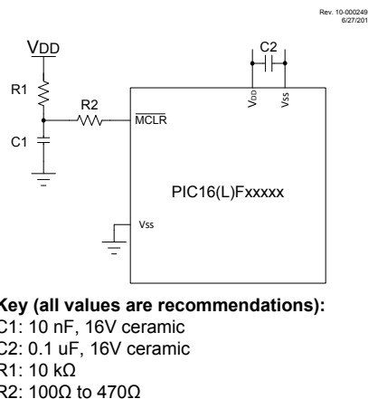
Figure 2-1. Recommended Minimum Connections
