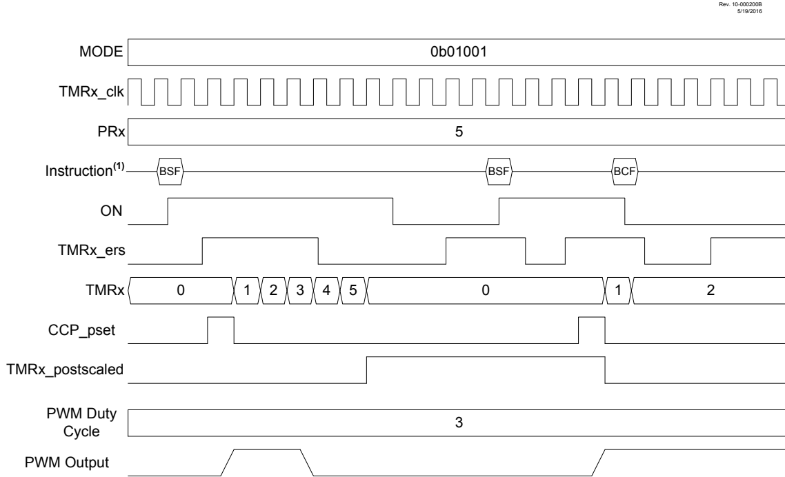
Figure 26-8. Edge-Triggered One-Shot Mode Timing Diagram (MODE = 01001)
