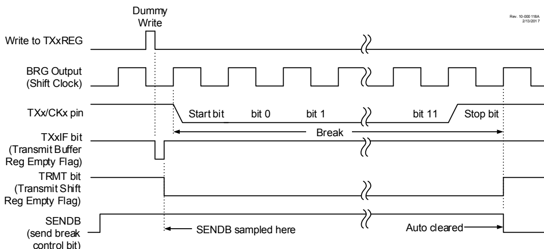
Figure 36-10. Send Break Character Sequence
