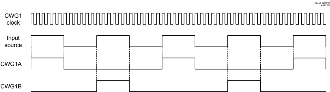
Figure 31-3. CWG Push-Pull Mode Operation
