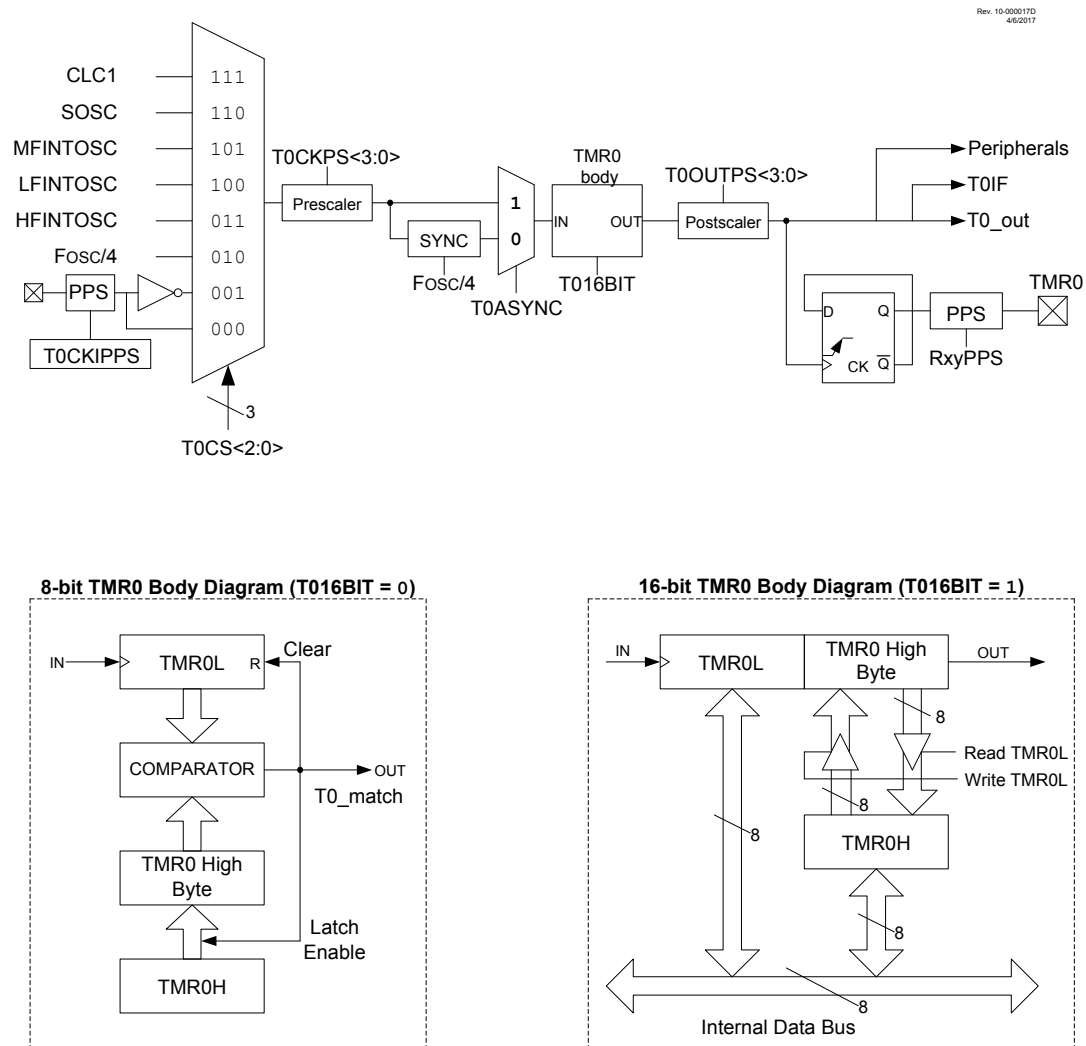
Figure 24-1. Timer0 Block Diagram
