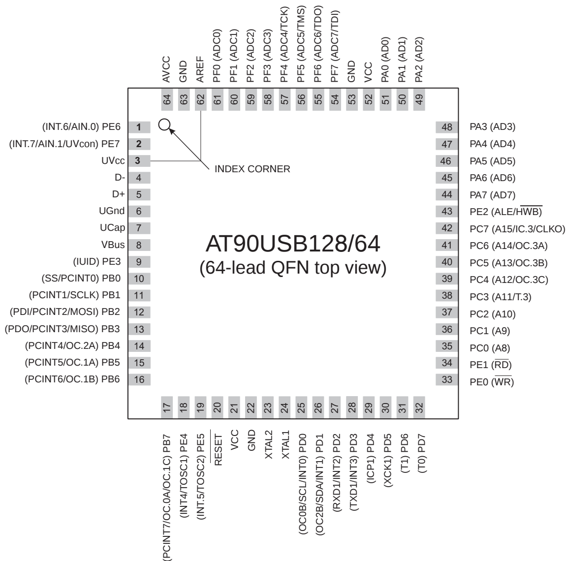
Figure 1-2. Pinout AT90USB64/128-QFN
