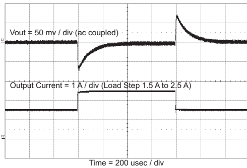
Figure 50. Load Transient
