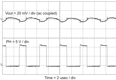
Figure 52. Output Ripple, CCM
