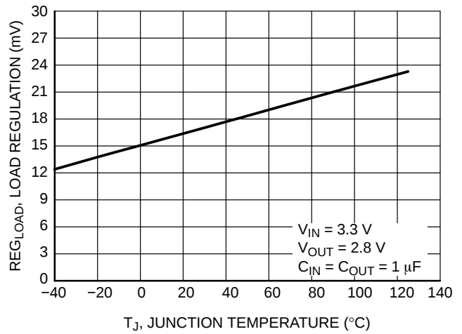
Figure 10. Load Regulation vs. Temperature V_{OUT} = 2.8 \text{ V}
