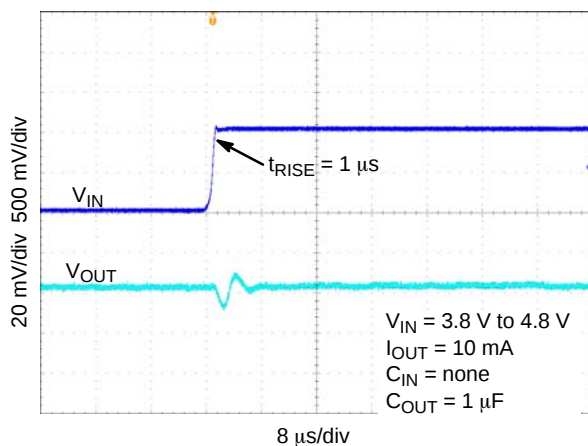
Figure 30. Line Transient Response – Rising Edge, V_{OUT} = 3.3 \text{ V} , I_{OUT} = 10 \text{ mA}
