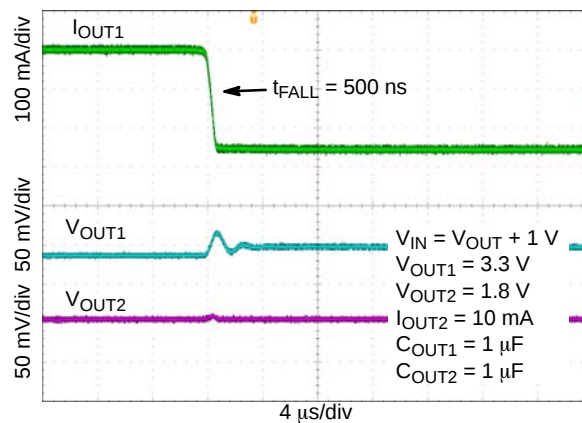
Figure 41. Load Transient Response – Falling Edge, I_{OUT} = 300 mA to 50 mA
