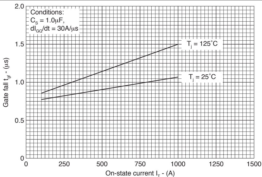
Fig.20 Gate fall time vs on-state current
