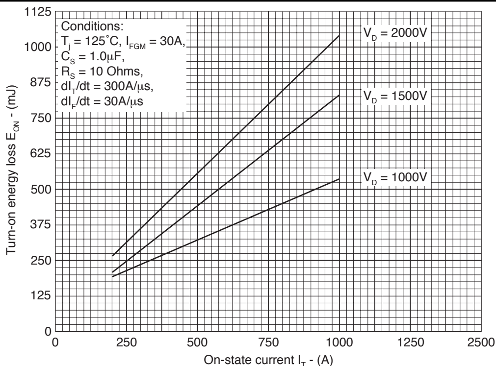
Fig.10 Turn-on energy vs on-state current
