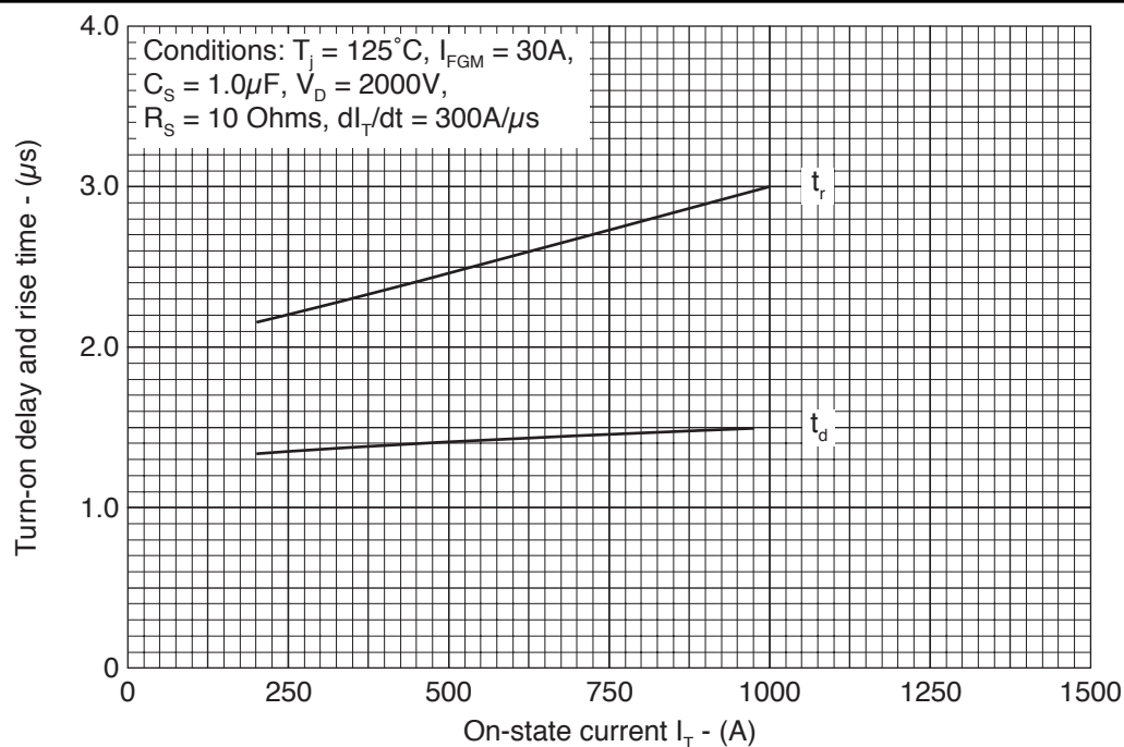
Fig.13 Delay time & rise time vs turn-on current
