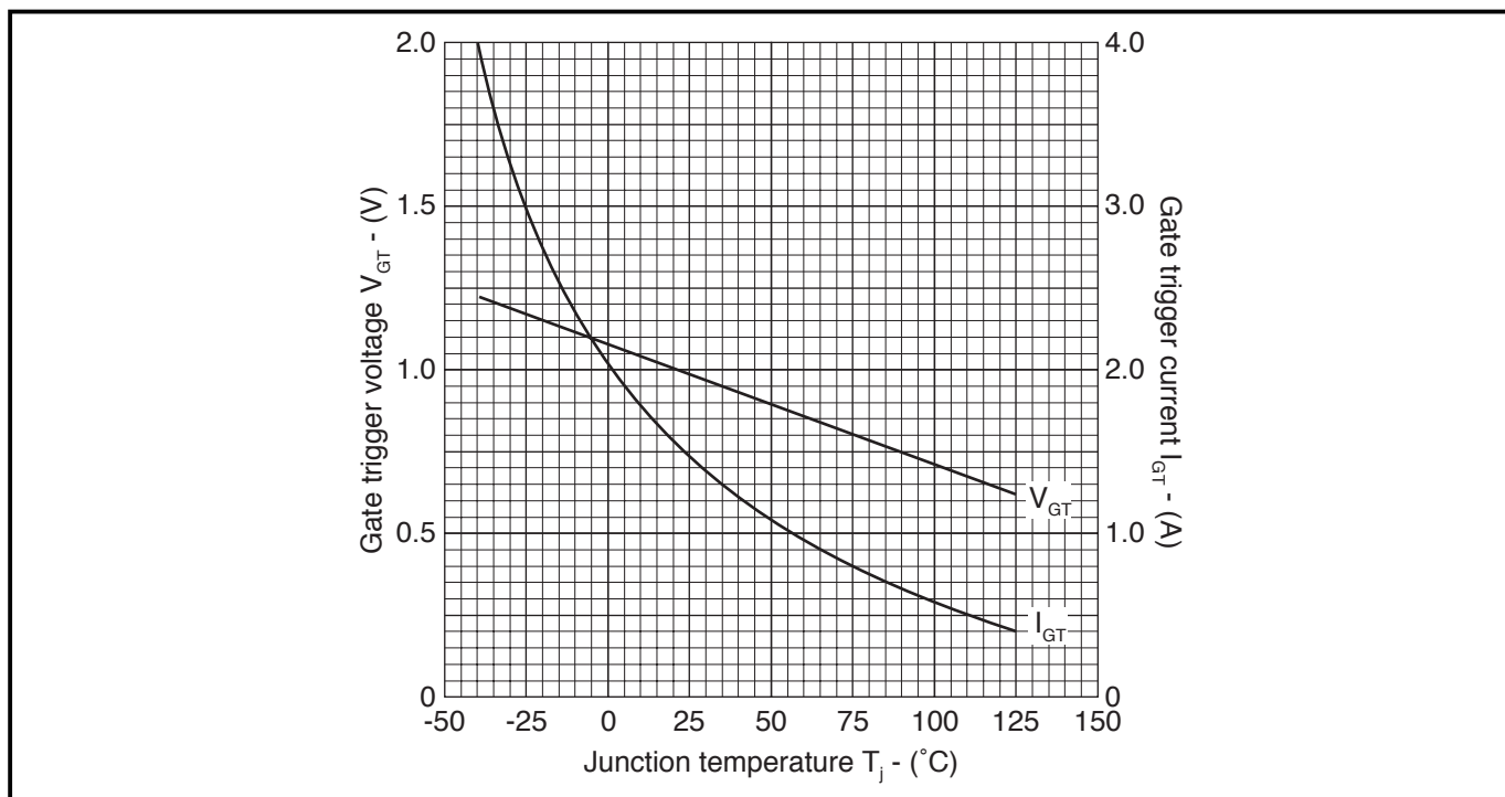
Fig.1 Maximum gate trigger voltage/current vs junction temperature
