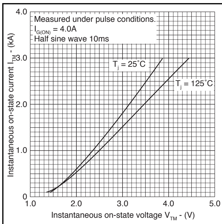
Fig.2 On-state characteristics
