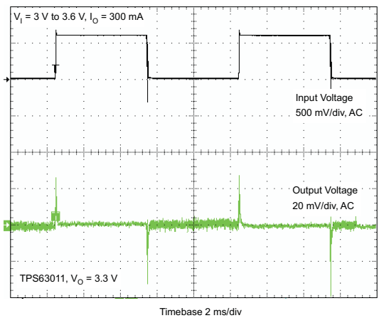
Figure 30. Line Transient Response (TPS63011)
