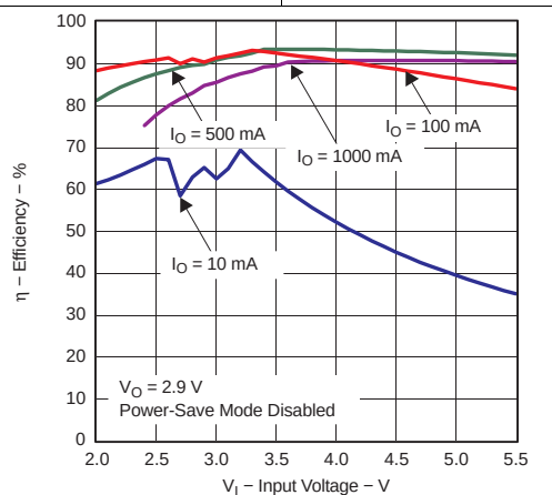
Figure 19. Efficiency vs Input Voltage (TPS63012)
