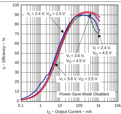
Figure 5. Efficiency vs Output Current (TPS63010)
