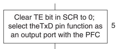
Figure 15.11 Sample Flowchart for Transmitting Multiprocessor Serial Data
