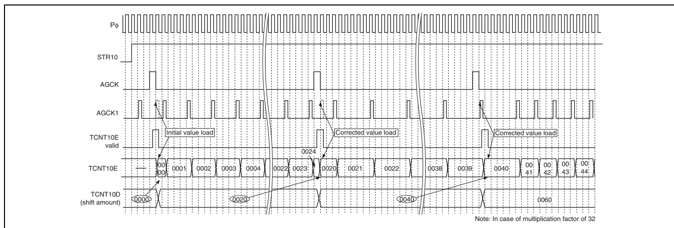
Figure 11.33 TCNT10E Operation
