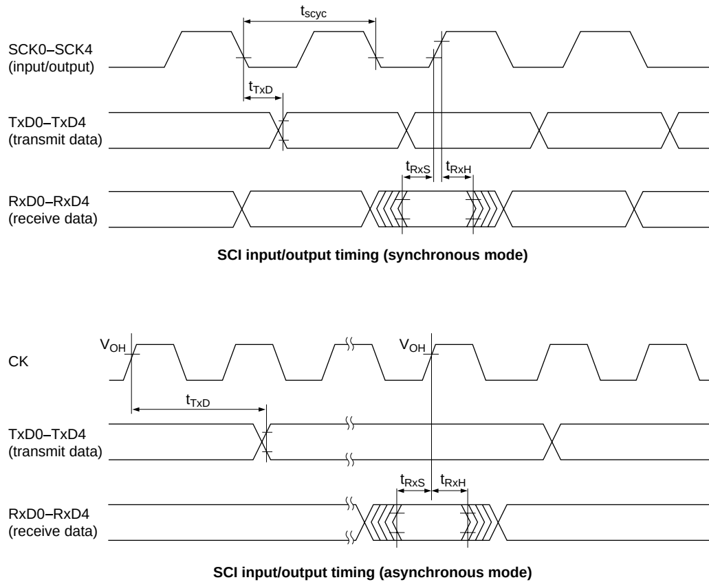
Figure 29.17 SCI Input/Output Timing
