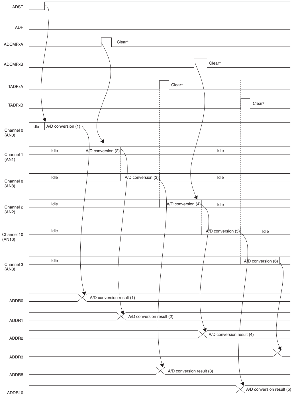
Figure 19.2 Example of Multi-Trigger A/D Converter Operation
