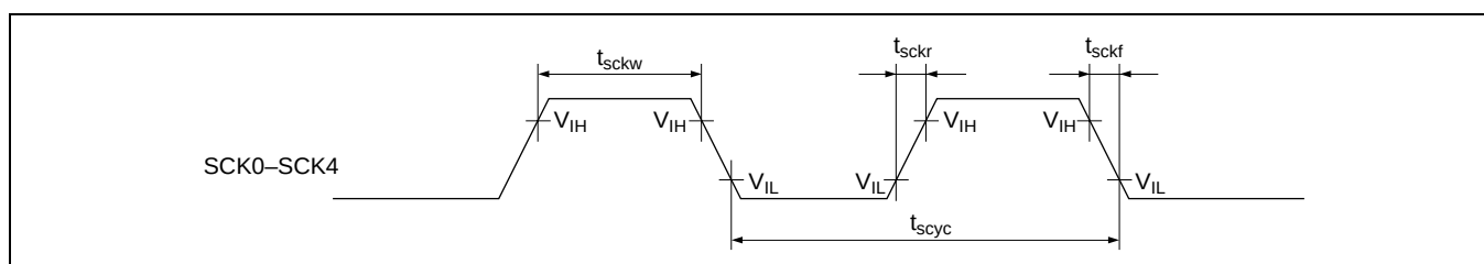
Figure 29.16 SCI Input/Output Timing
