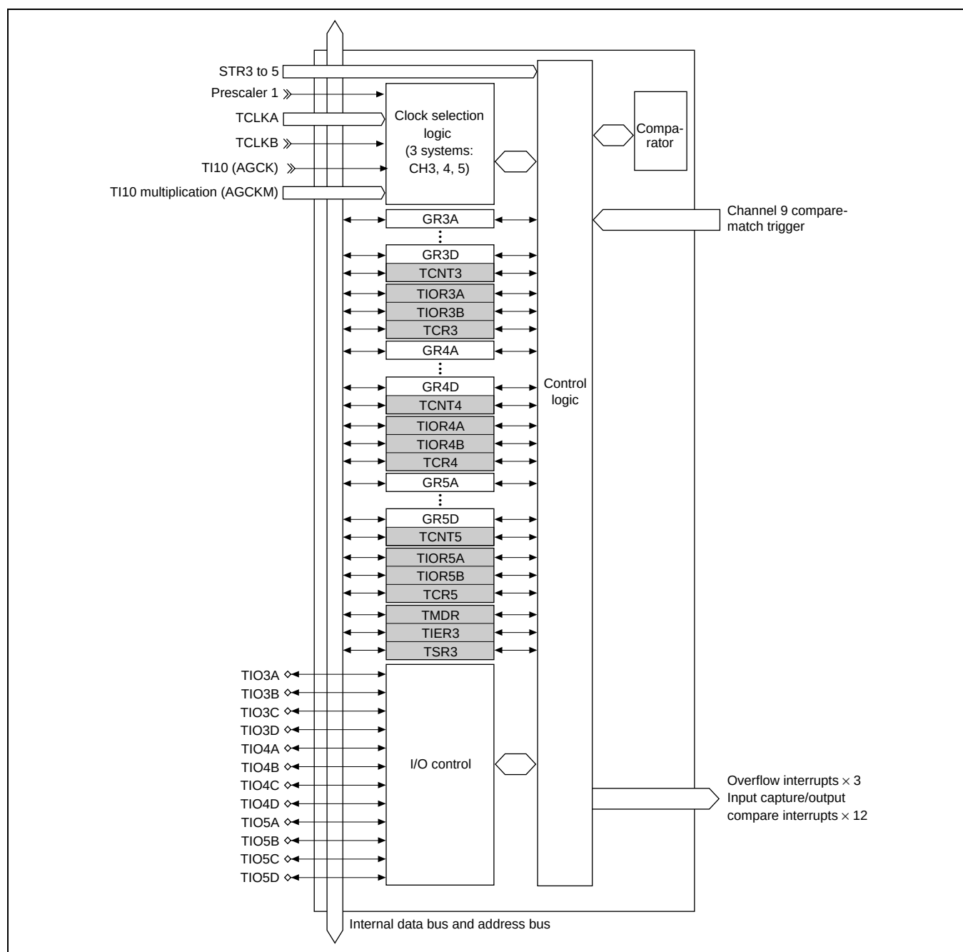
Figure 11.5 Block Diagram of Channels 3 to 5
