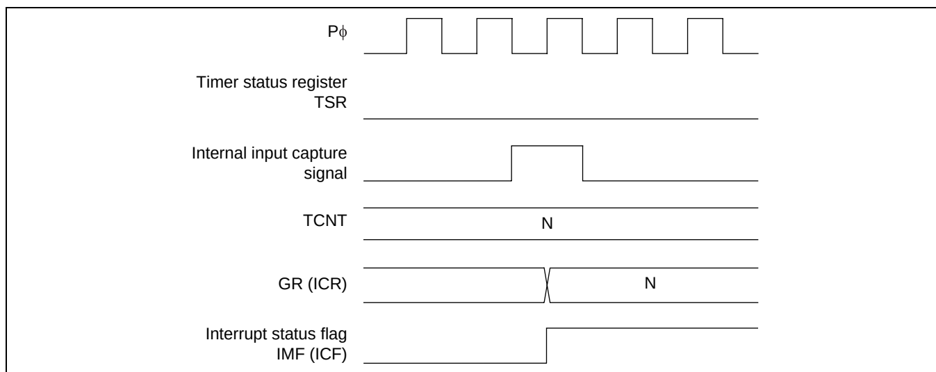
Figure 11.71 Input Capture Operation before Free-Running Counter is Started
