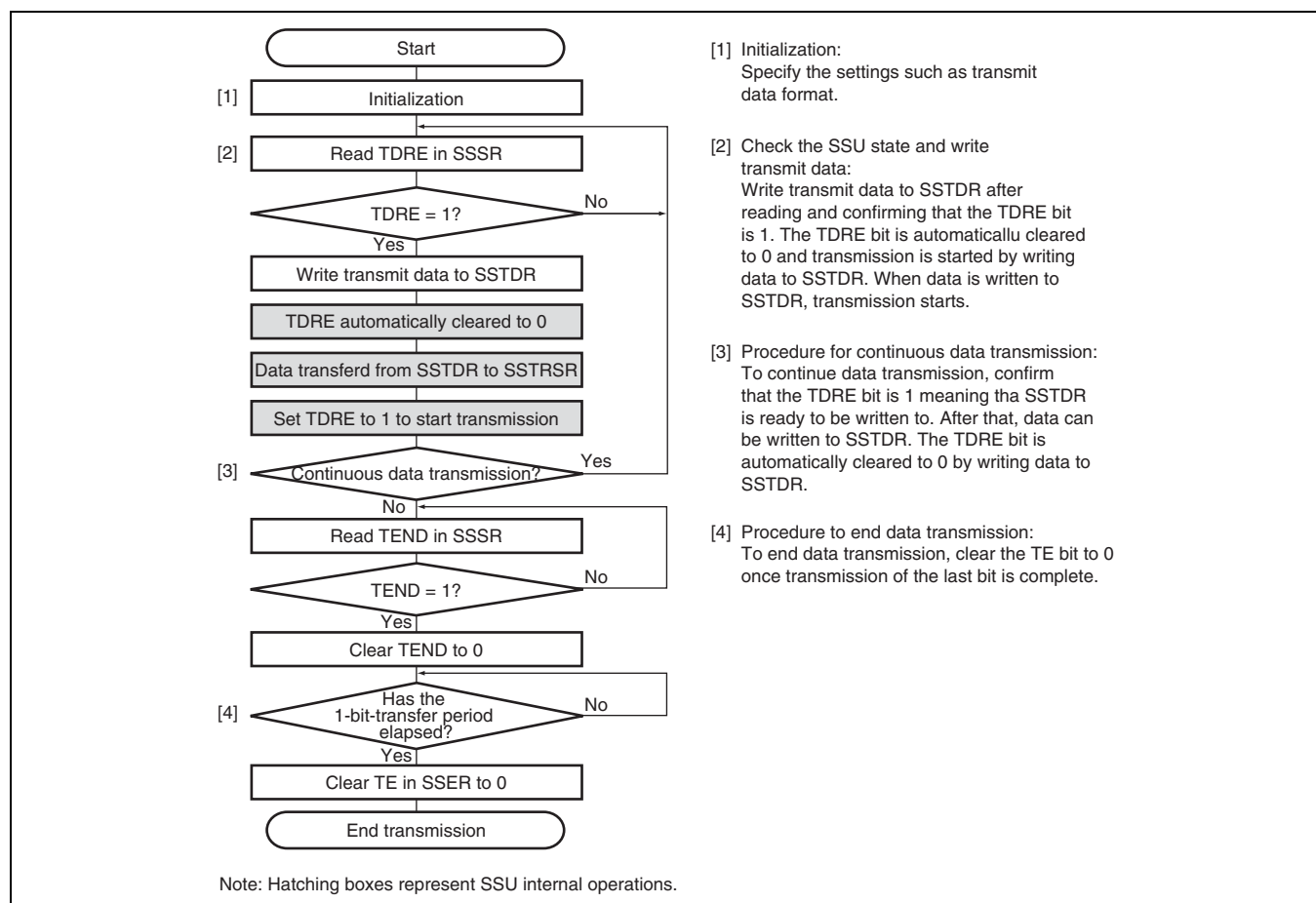
Figure 16.6 Example of Data Transmission Flowchart
