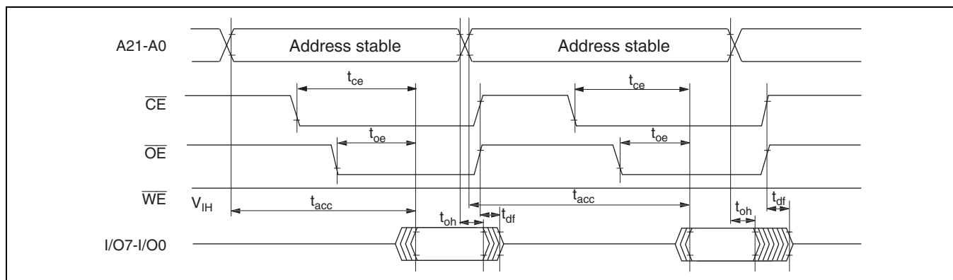
Figure 25.35 \overline{\text{CE}}/\overline{\text{OE}} Clock Read
