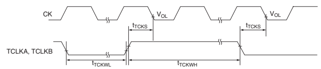
Figure 29.13 ATU Clock Input Timing
