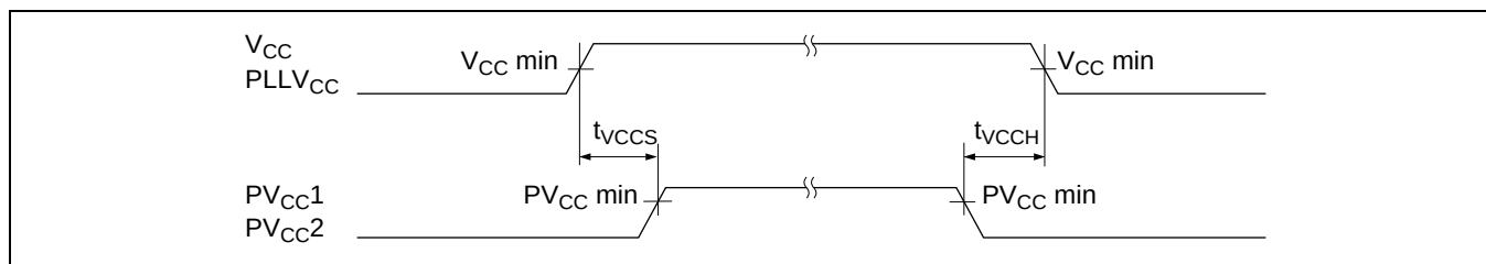
Figure 29.1 Power-On/Off Timing
