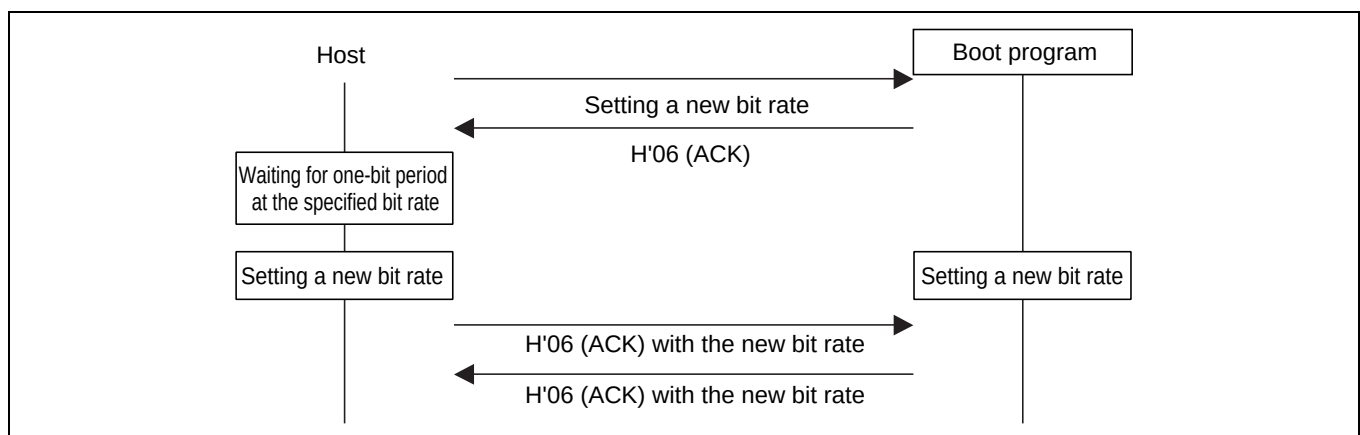
Figure 25.29 New Bit-Rate Selection Sequence
