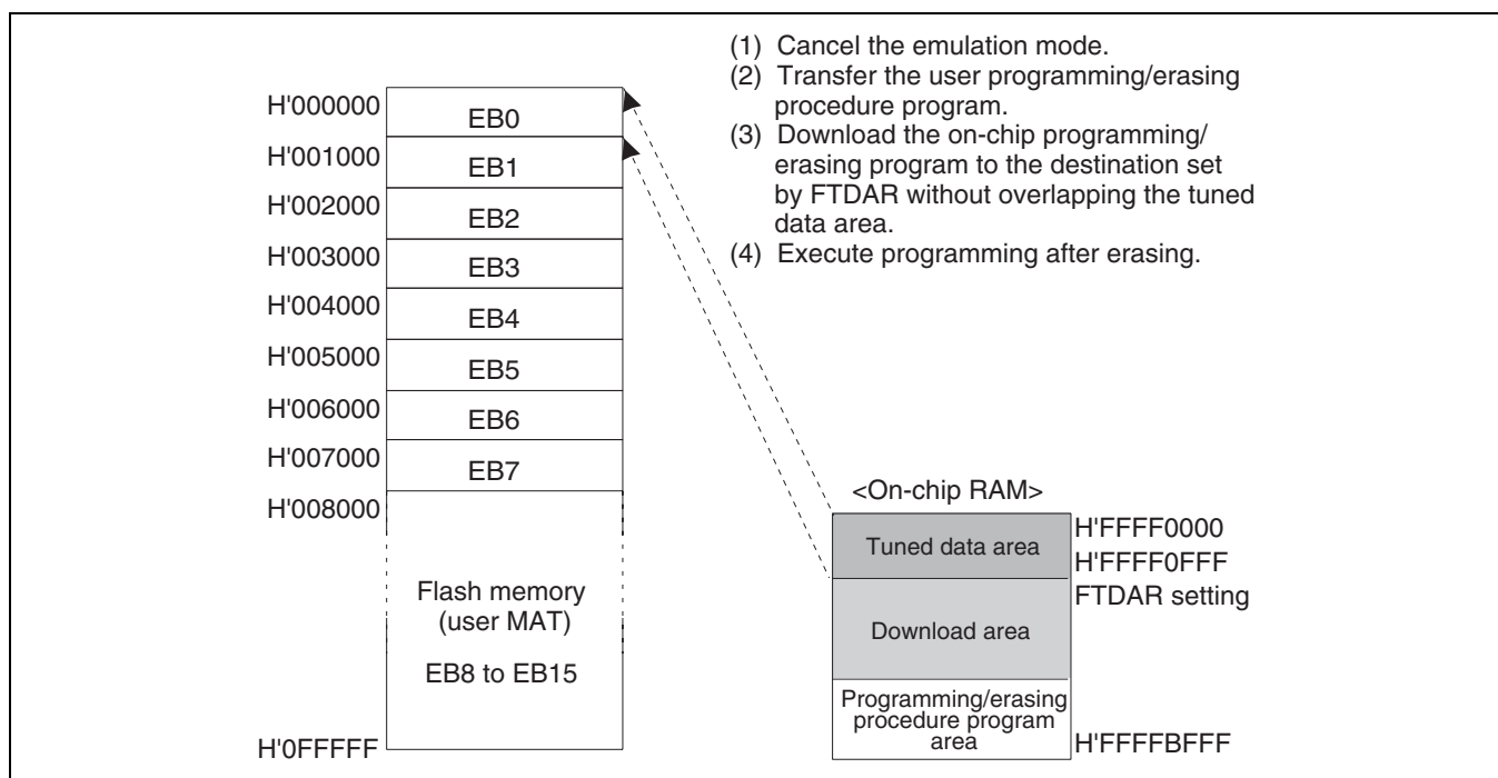
Figure 24.19 Programming of Tuned Data
