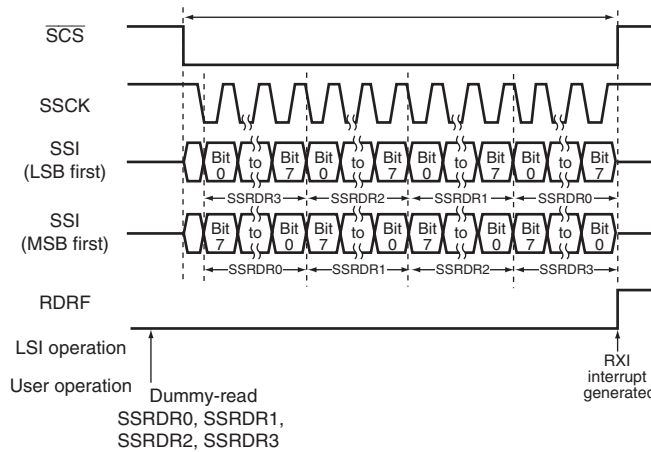
Figure 16.7 Example of Reception Operation
