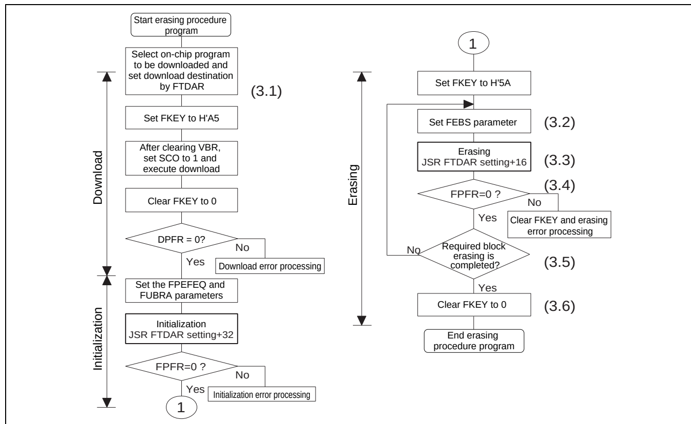
Figure 24.12 Erasing Procedure
