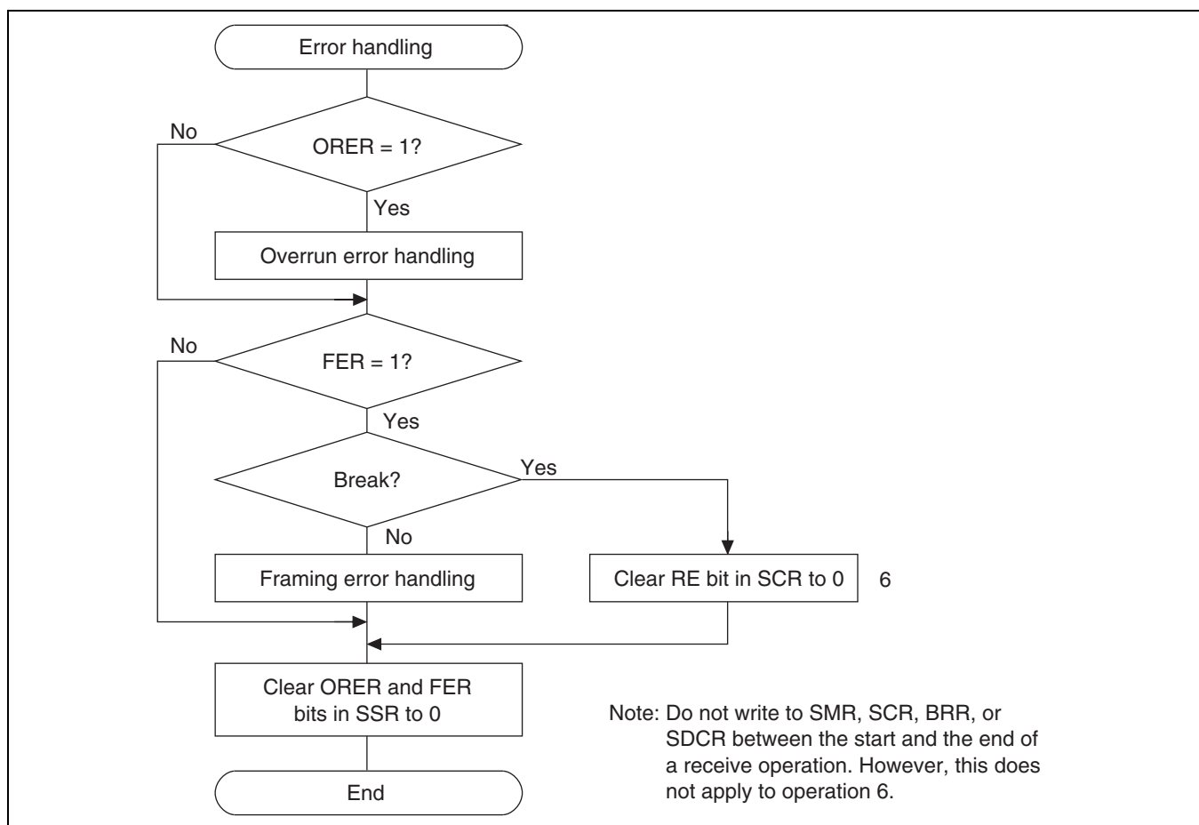
Figure 15.14 Sample Flowchart for Receiving Multiprocessor Serial Data (2)
