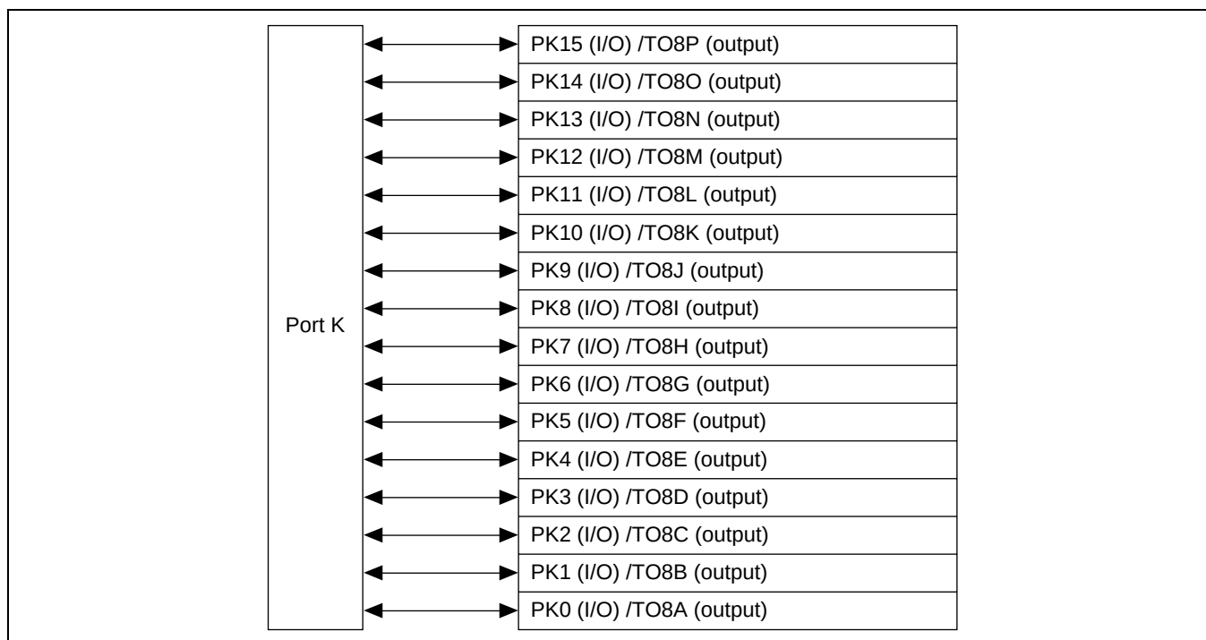
Figure 23.10 Port K
