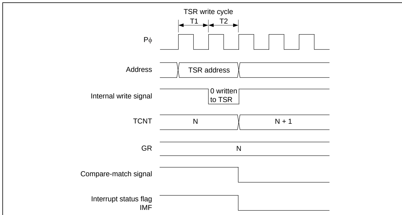
Figure 11.67 Contention between Interrupt Status Flag Setting by Compare-Match and Clearing
