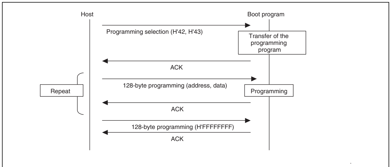
Figure 25.30 Programming Sequence
