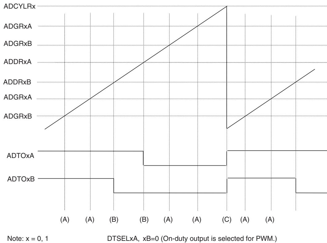
Figure 19.4 Example of Output Waveform from MTAD PWM
