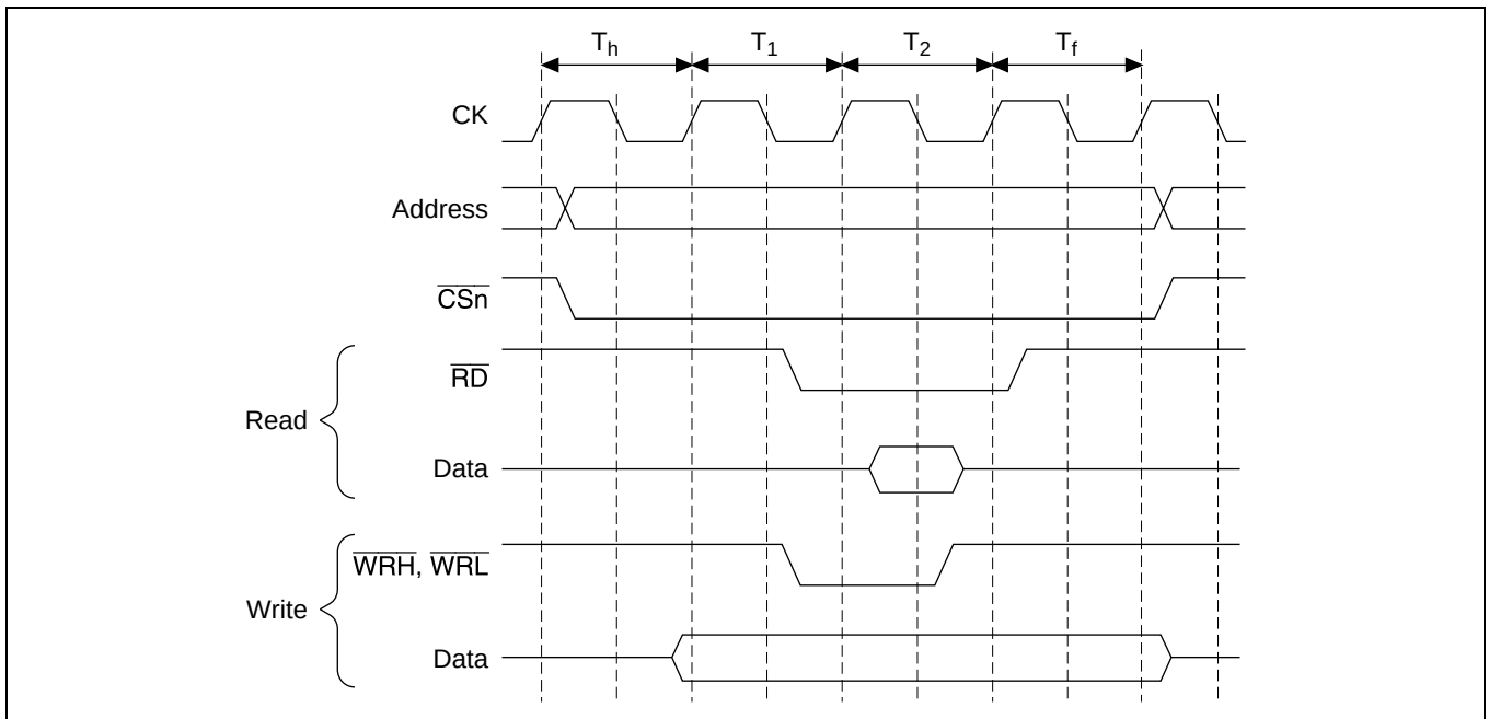
Figure 9.6 \overline{\text{CS}} Assert Period Extension Function
