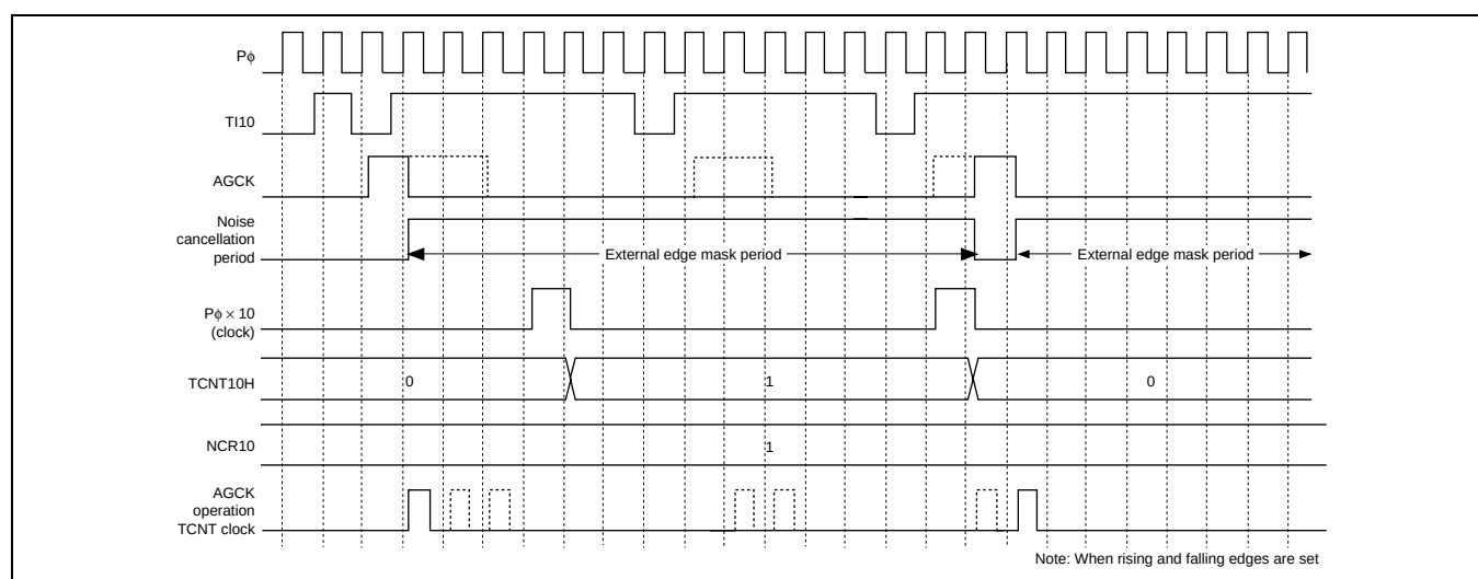
Figure 11.27 Edge Input Operation (With Noise Cancellation)
