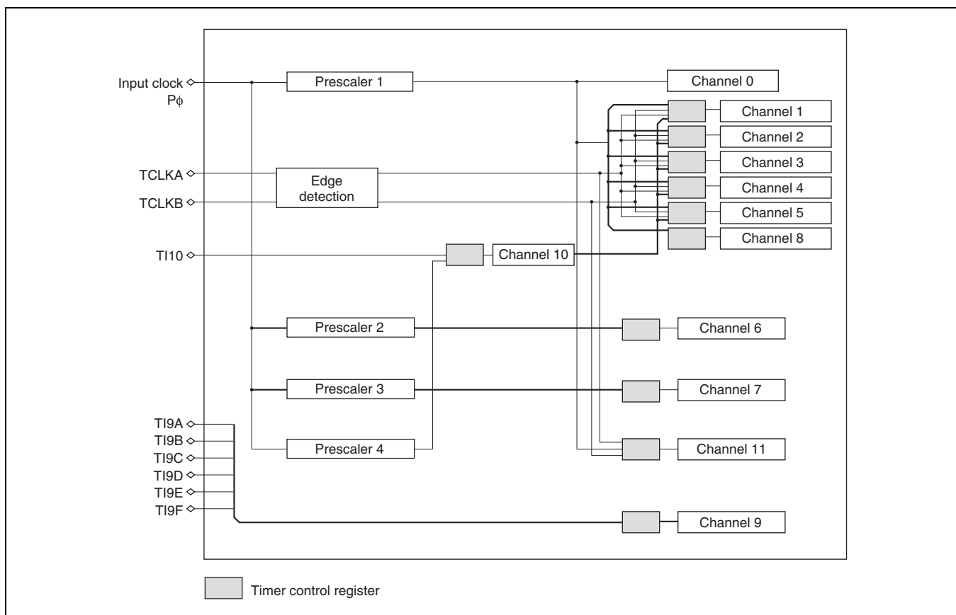
Figure 11.12 Prescaler Diagram
