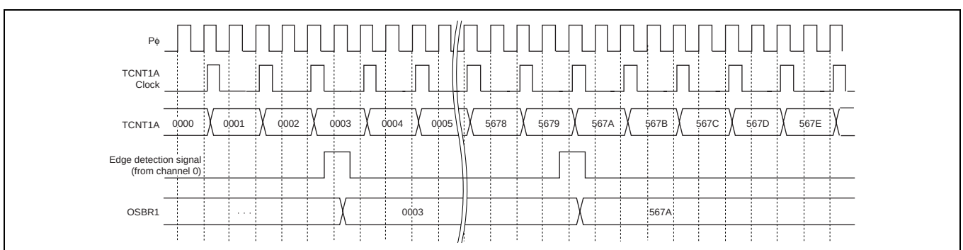
Figure 11.20 Twin-Capture Operation
