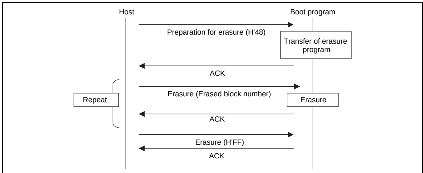
Figure 25.31 Erasing Sequence
