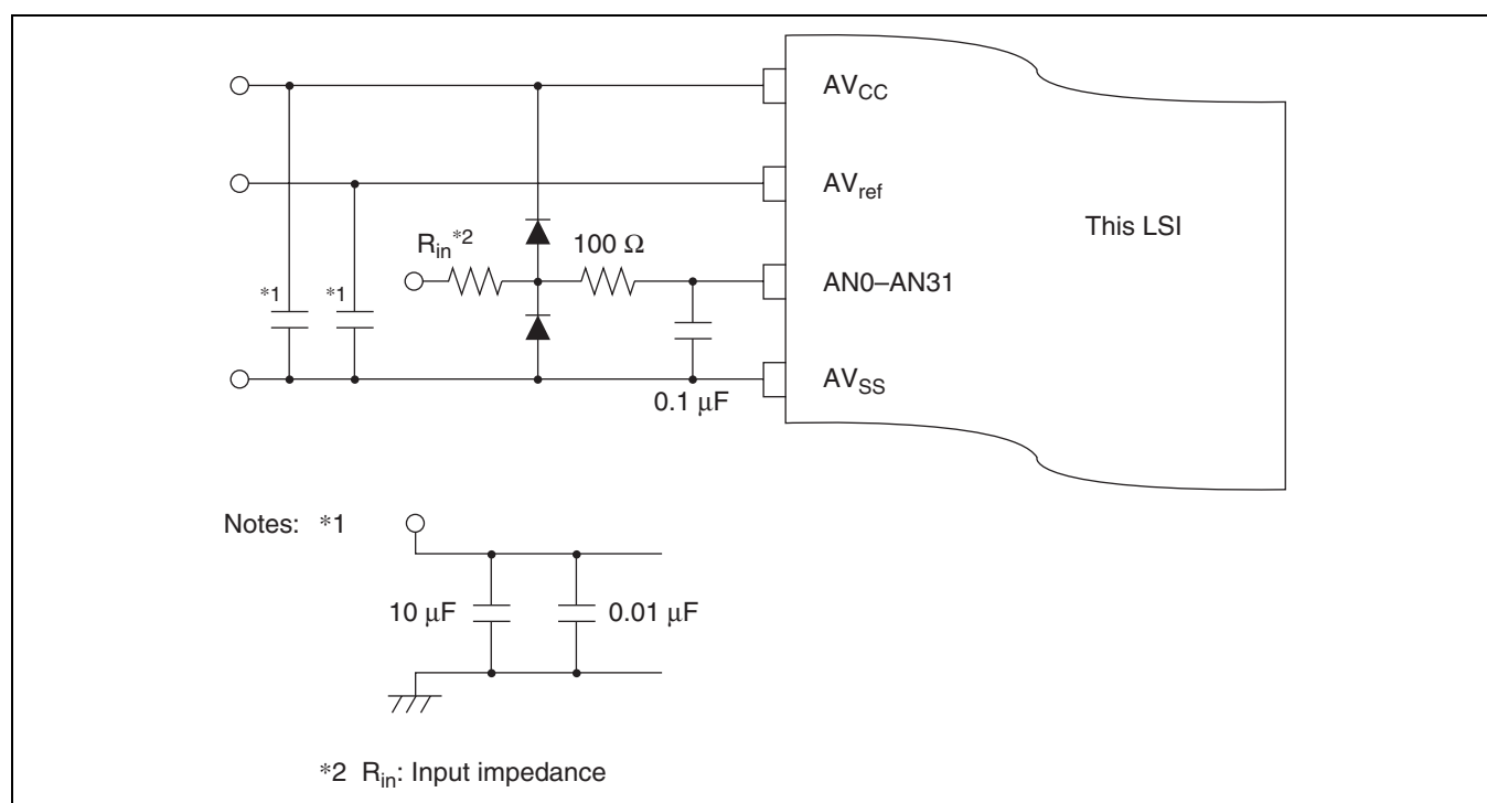
Figure 18.9 Example of Analog Input Pin Protection Circuit
