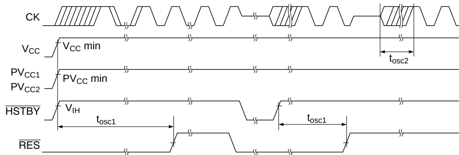
Figure 29.4 Oscillation Settling Time
