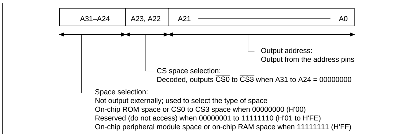
Figure 9.2 Address Format
