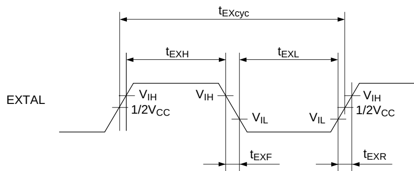
Figure 29.2 Peripheral Clock Timing
