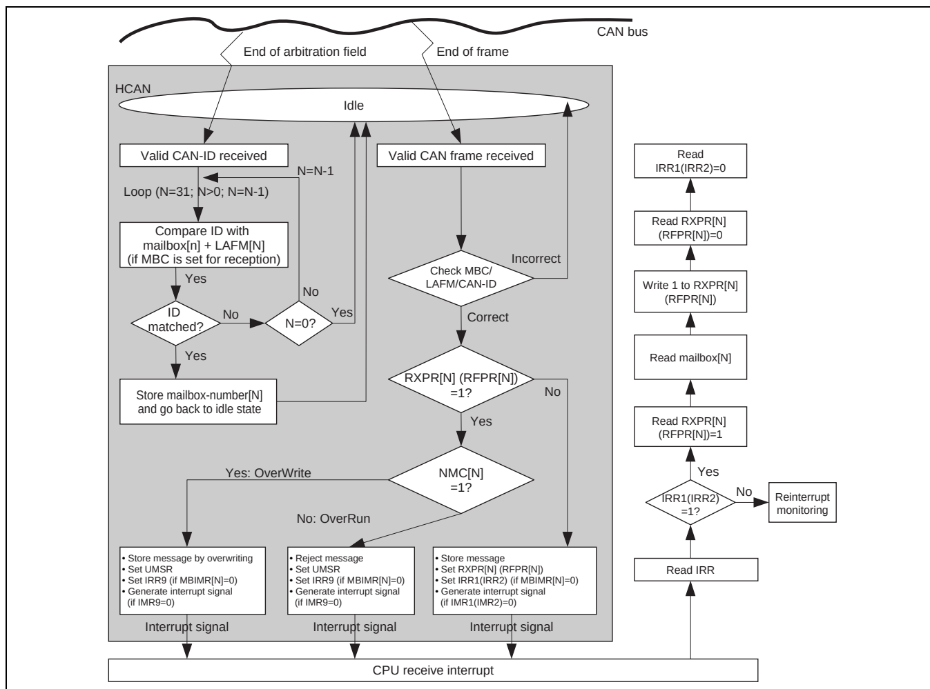
Figure 17.11 Message Receive Sequence
