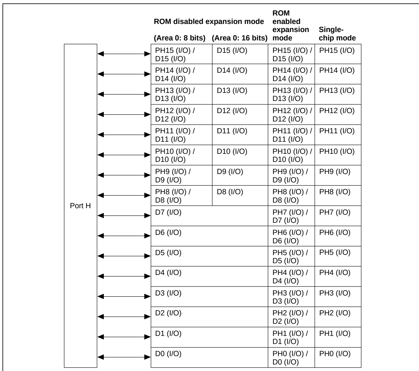
Figure 23.8 Port H
