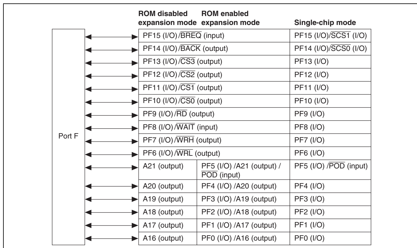
Figure 23.6 Port F
