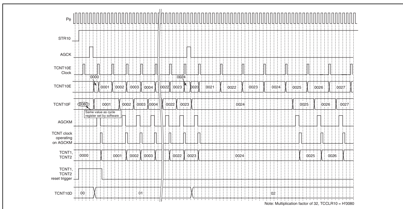
Figure 11.34 TCNT10F Operation (At Startup)
