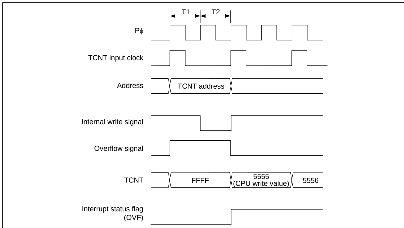
Figure 11.66 Contention between TCNT Write and Overflow
