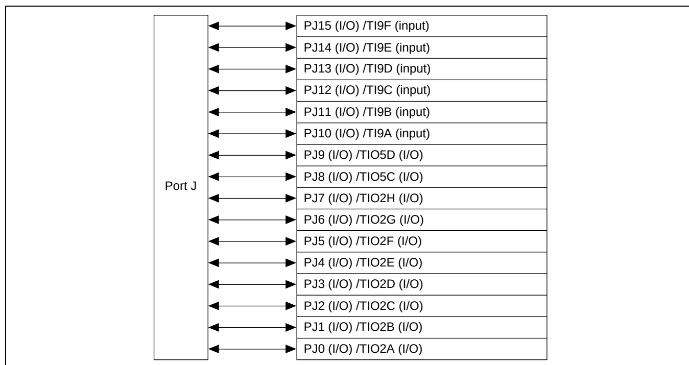
Figure 23.9 Port J
