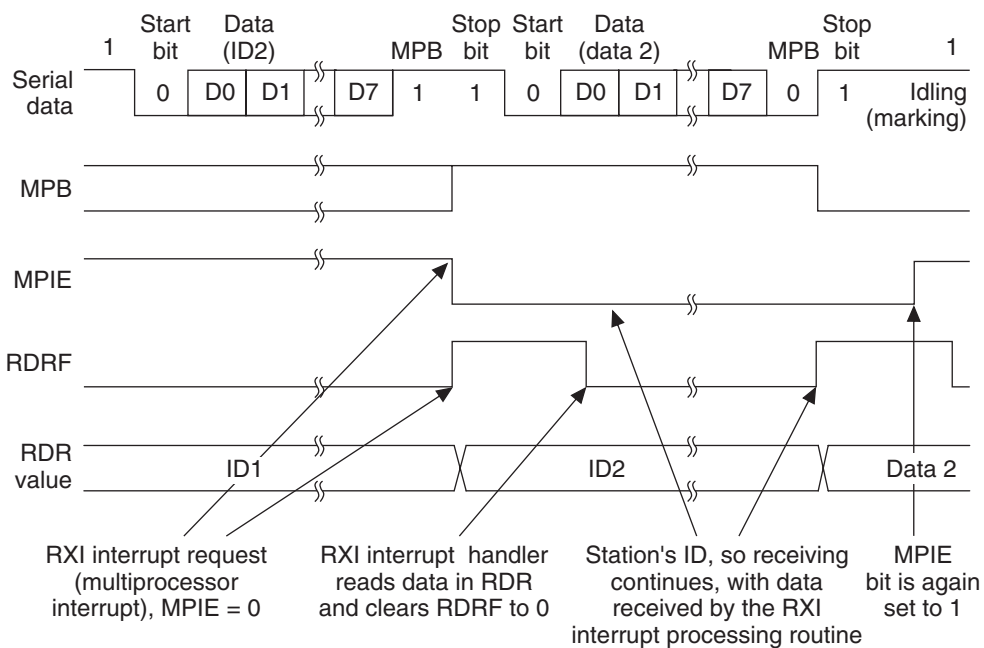
(B) ID Matches
