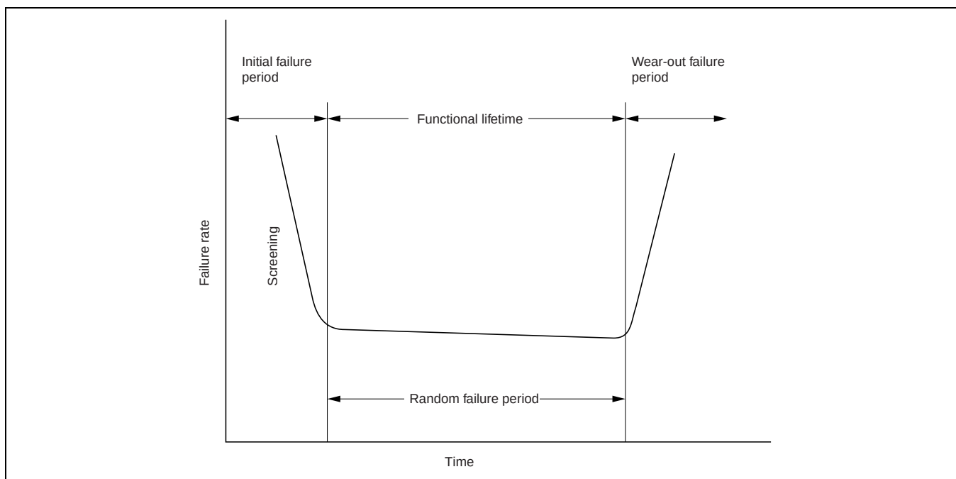
Figure 28.1 Failure Rate Curve (Bathtub Curve)
