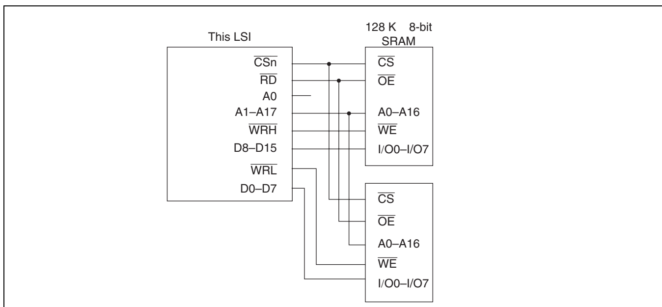
Figure 9.13 Example of 16-Bit Data Bus Width SRAM Connection
