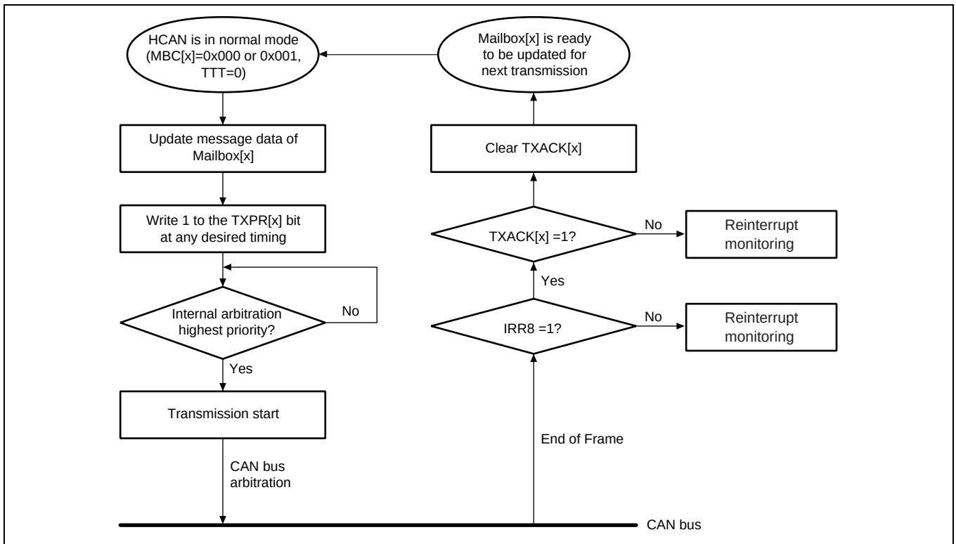
Figure 17.8 Transmission Request
