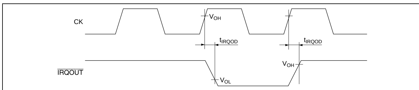
Figure 29.7 Interrupt Signal Output Timing
