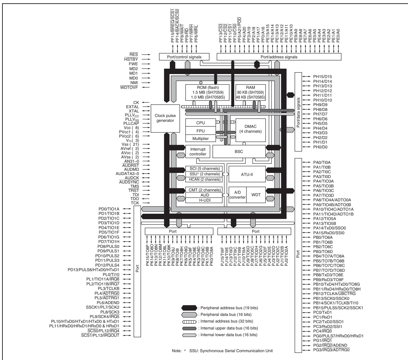
Figure 1.1 Block Diagram
