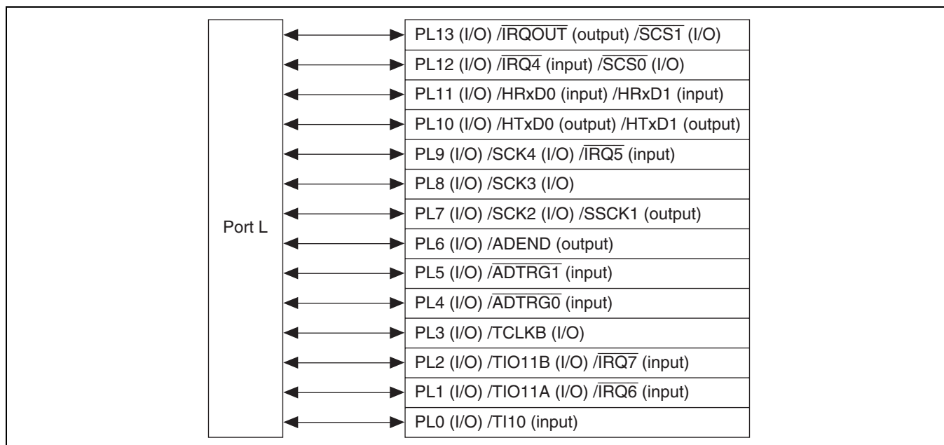
Figure 23.11 Port L
