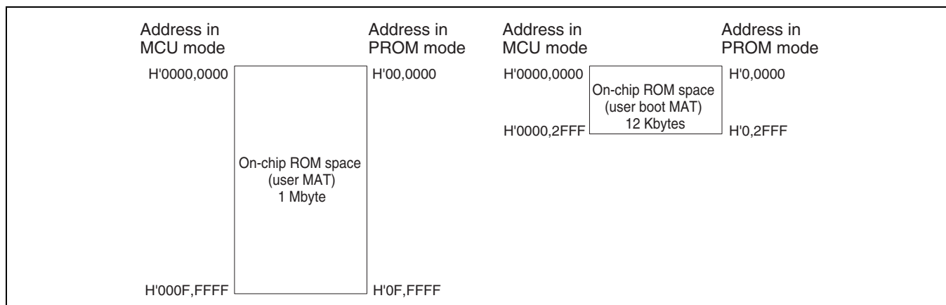
Figure 24.24 Mapping of On-Chip Flash Memory
