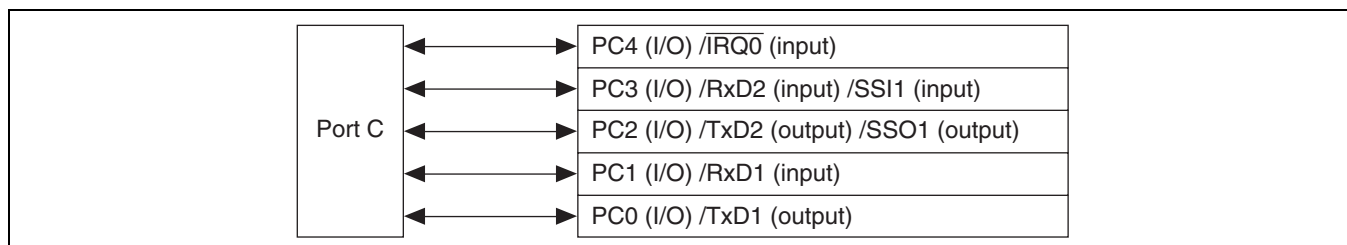
Figure 23.3 Port C
