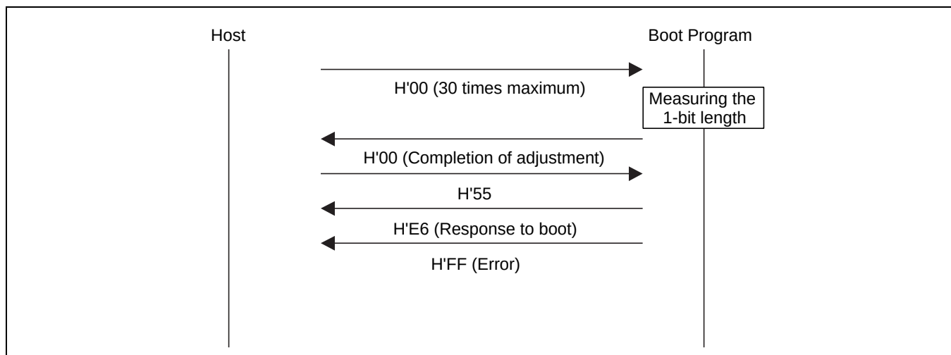
Figure 25.27 Bit-Rate-Adjustment Sequence
