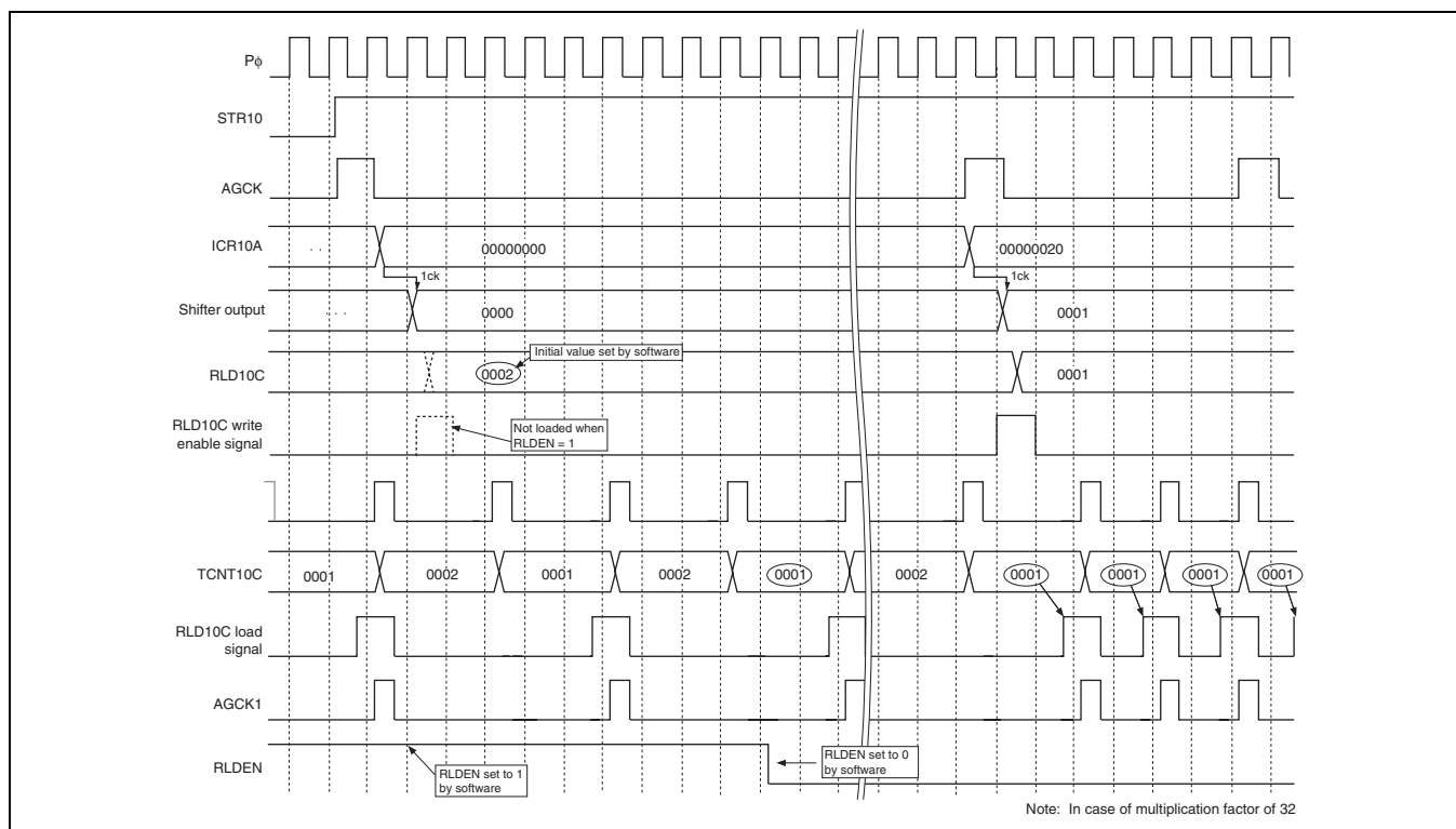
Figure 11.30 TCNT10C Operation
