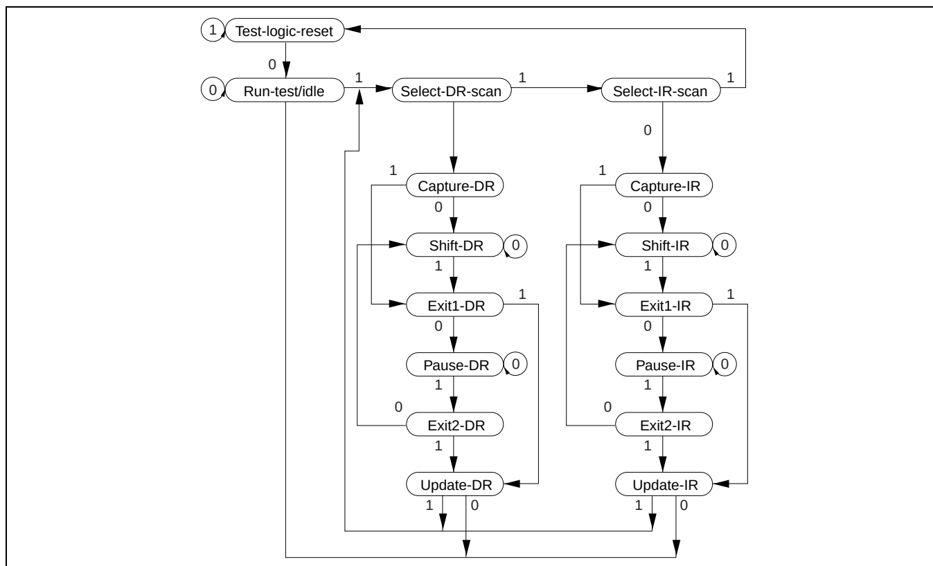
Figure 20.2 TAP Controller State Transitions
