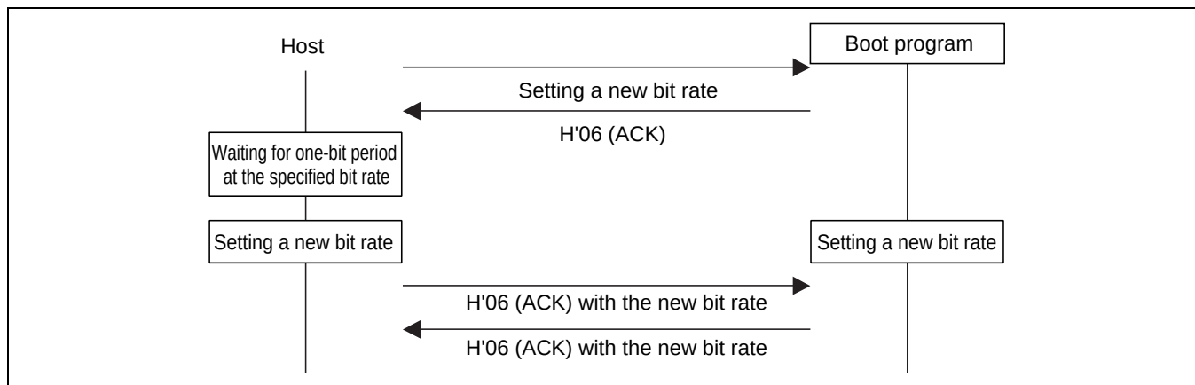
Figure 24.29 New Bit-Rate Selection Sequence
