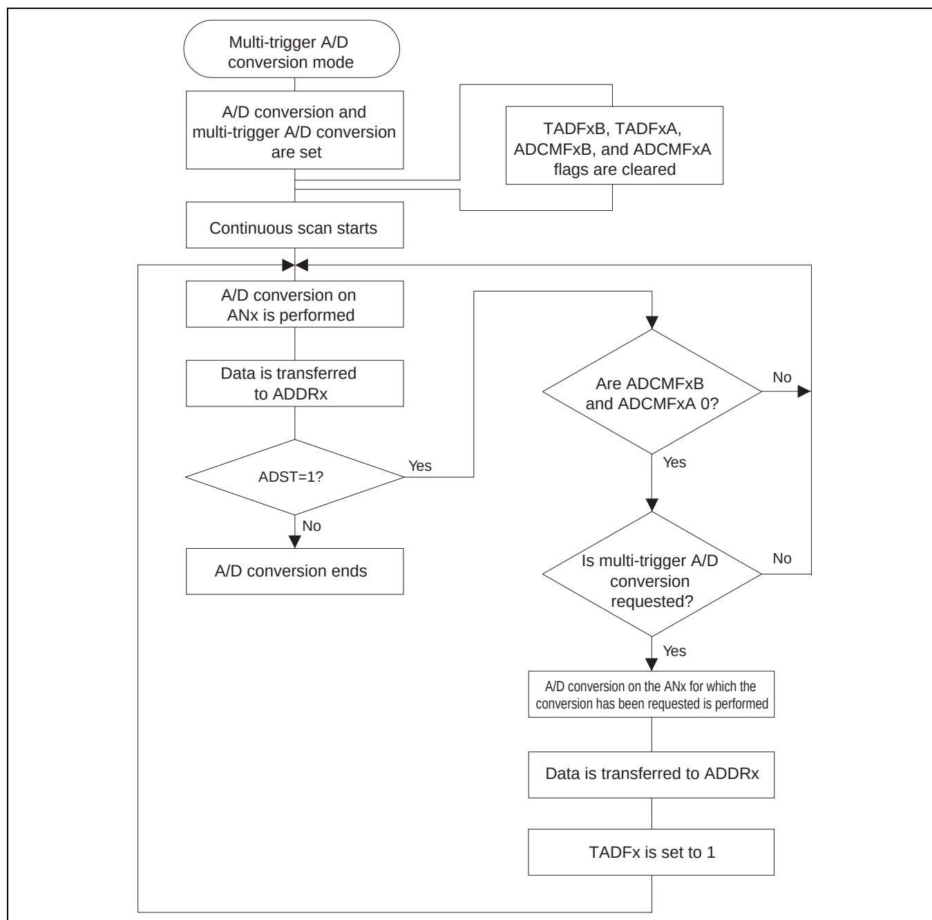
Figure 19.3 Flowchart of Multi-Trigger A/D Converter Operation
