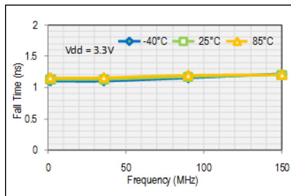
FIGURE 3-5: Fall Time.
