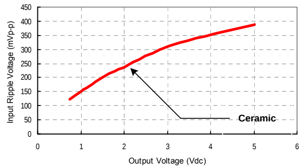
Figure 28: Input ripple voltage vs. output models, I_o = 20A ( C_{in} = 4x22uF ceramic capacitors at the input)
