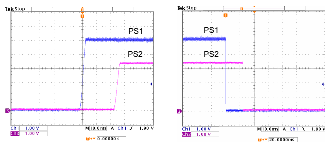
Figure 35: Sequential start-up
