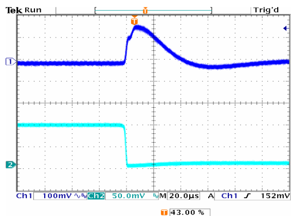
Figure 16: Typical transient response to step load change at 5\text{A}/\mu\text{s} from 100% to 50% of I_o , max at 12Vin, 0.75V out ( C_{out} = 1\mu\text{F} + 100\mu\text{F} ceramic, 470 \mu\text{F} poscap).
