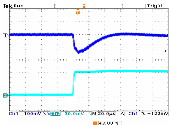
Figure 17: Typical transient response to step load change at 5\text{A}/\mu\text{s} from 50% to 100% of I_o , max at 12Vin, 1.2V out ( C_{out} = 1\mu\text{F} + 100\mu\text{F} ceramic, 470 \mu\text{F} poscap).
