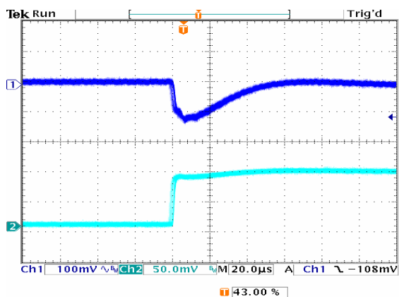
Figure 15: Typical transient response to step load change at 5\text{A}/\mu\text{s} from 50% to 100% of I_o , max at 12Vin, 0.75V out ( C_{out} = 1\mu\text{F} + 100\mu\text{F} ceramic, 470 \mu\text{F} poscap).
