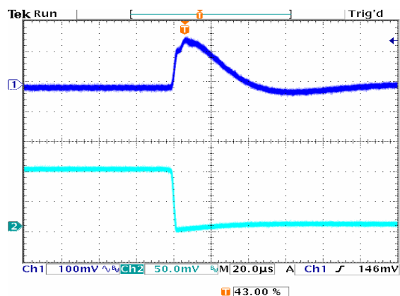
Figure 18: Typical transient response to step load change at 5\text{A}/\mu\text{s} from 100% to 50% of I_o , max at 12Vin, 1.2V out ( C_{out} = 1\mu\text{F} + 100\mu\text{F} ceramic, 470 \mu\text{F} poscap).
