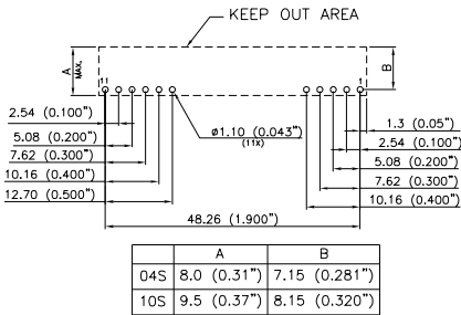
RECOMMENDED P.W.B. PAD LAYOUT
