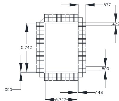
SOLDER MASK
