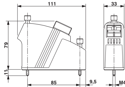
Dimensioned drawing
