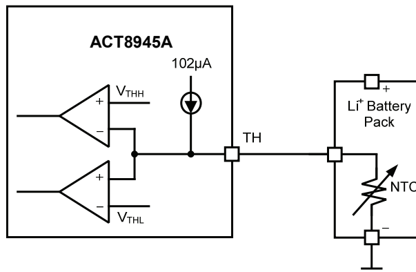
Figure 7: Simple Configuration
