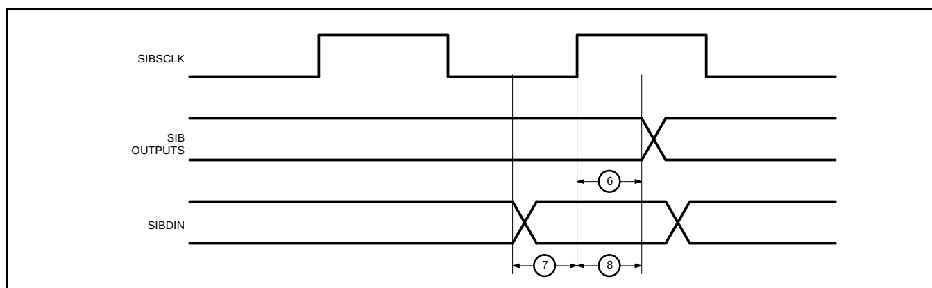
Figure 13. SIB Timing
