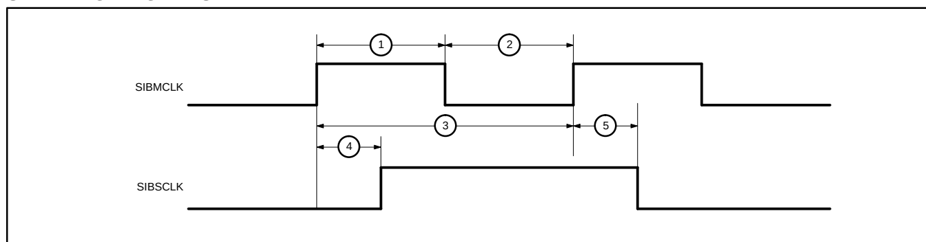
Figure 12. SIB CLK Timing
