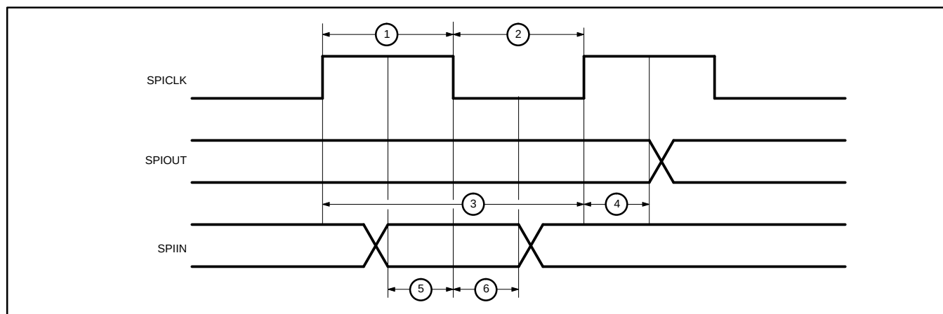
Figure 14. SPI Timing (PHAPOL = 1)
