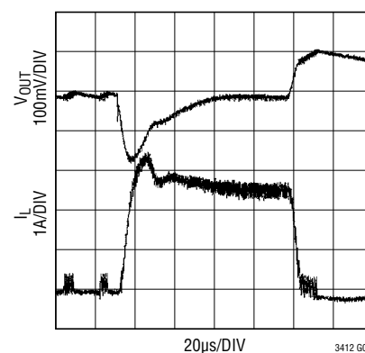
Load Step Transient Burst Mode Operation
