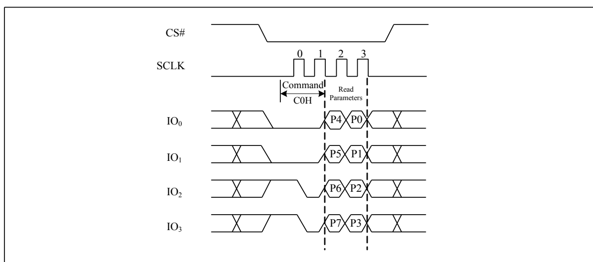
Figure 39. Set Read Parameters command Sequence Diagram
