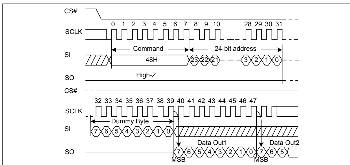
Figure 33. Read Security Registers command Sequence Diagram
