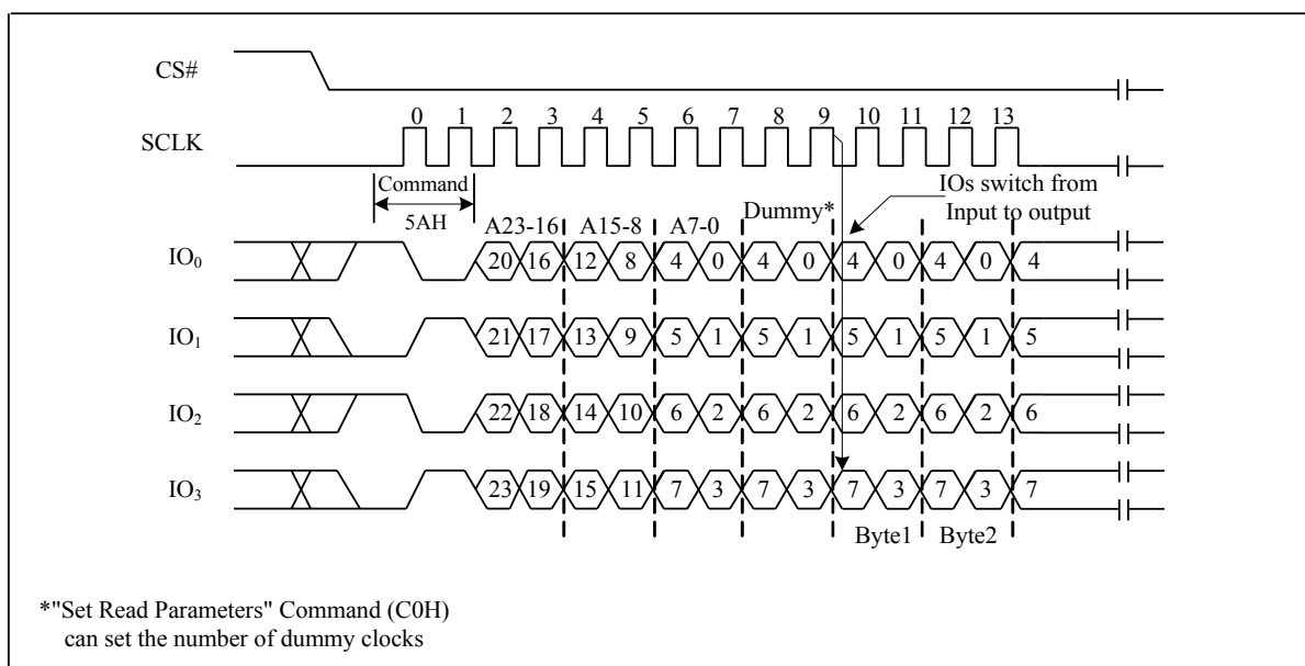
Figure 44a. Read Serial Flash Discoverable Parameter command Sequence Diagram (QPI)
