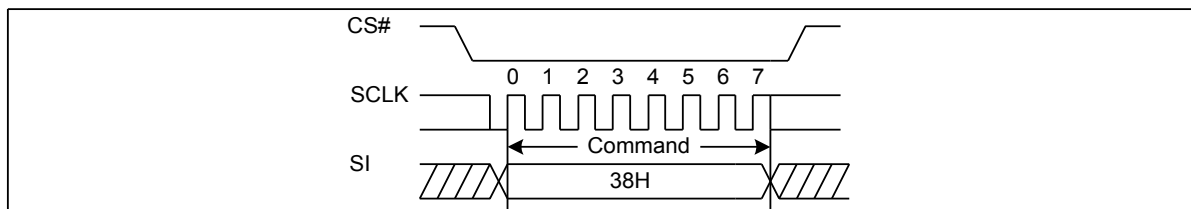
Figure 41. Enable QPI mode command Sequence Diagram
