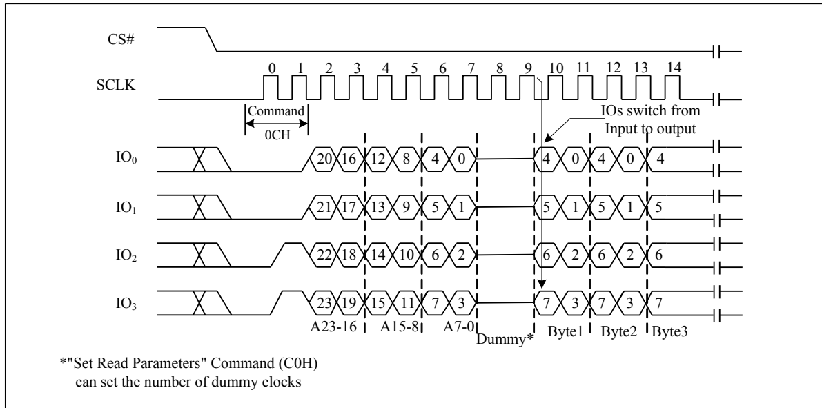
Figure 40. Burst Read with Wrap command Sequence Diagram
