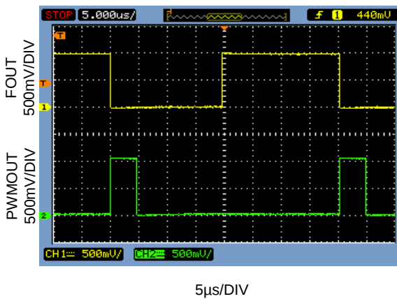
FOUT and PWMOUT Transient Response V_{DD} = 1V , V_{CNTRL} = 0.035 \times V_{DD} , C_{LOAD} = 22pF
