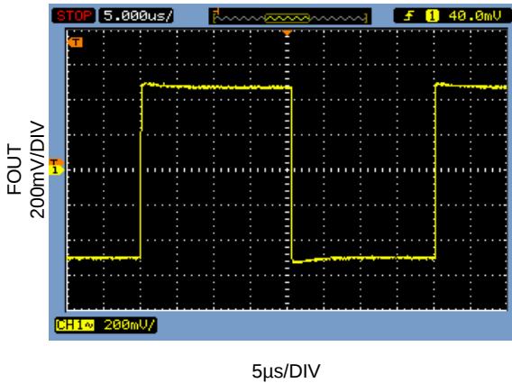
FOUT Transient Response V_{DD} = 1V , C_{LOAD} = 47pF
