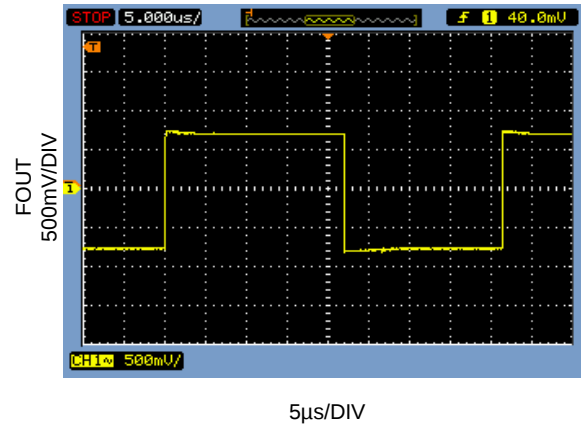
FOUT Transient Response V_{DD} = 1.5V , C_{LOAD} = 47pF
