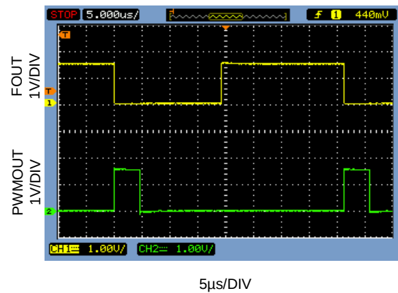
FOUT and PWMOUT Transient Response V_{DD} = 1.5V , V_{CNTRL} = 0.035 \times V_{DD} , C_{LOAD} = 22pF
