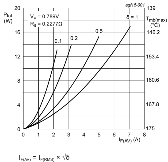
Fig. 1. Forward power dissipation as a function of average forward current; square wave pulse; typical values; per diode
