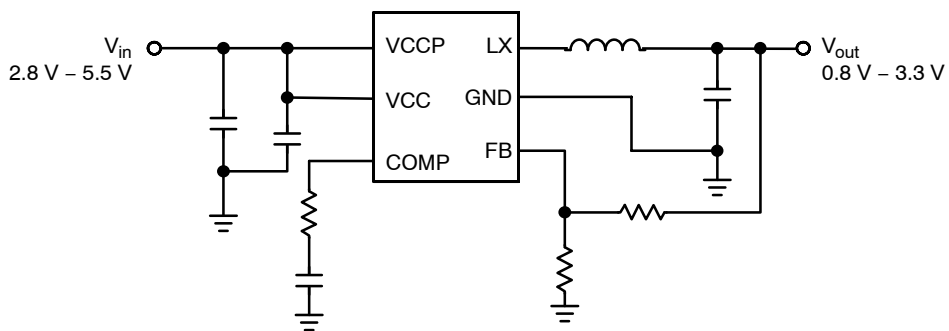
Figure 2. NCP1599 Application Circuit
