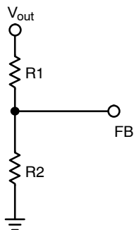
Figure 3. Output divider
