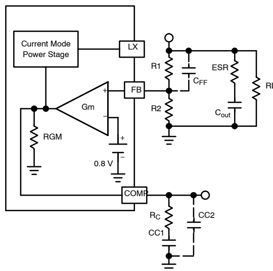
Figure 4. NCP1599 Compensation Components
