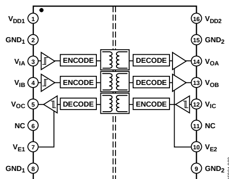
Figure 2. ADuM3301 Functional Block Diagram
