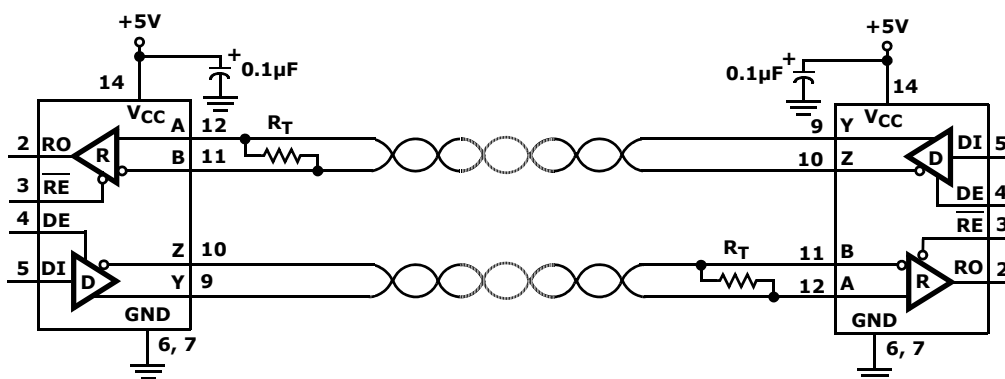
ISL3150E, ISL3153E, ISL3156E (SOIC PIN NUMBERS SHOWN)
