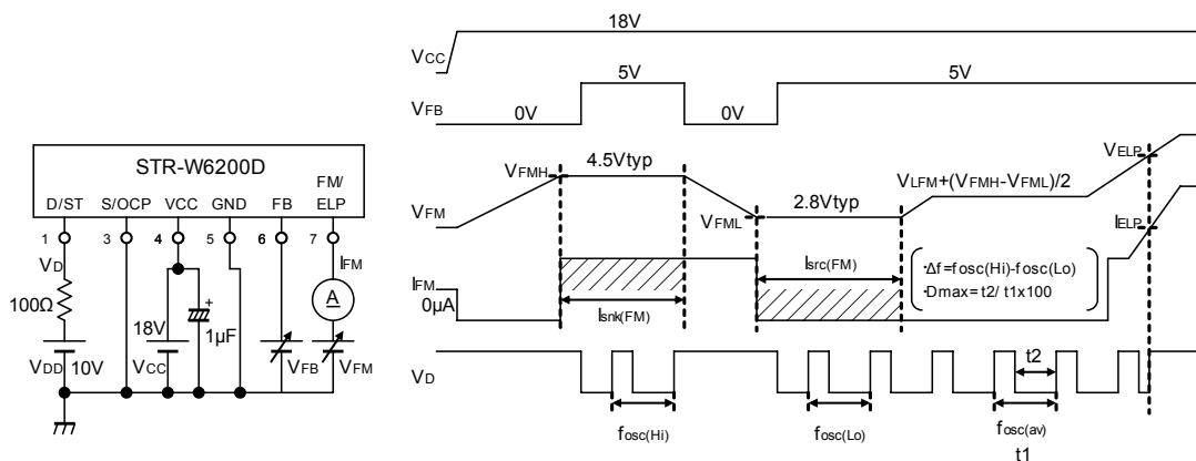
Measurement Circuit 3
