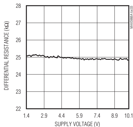
SIGNATURE RESISTANCE vs. SUPPLY VOLTAGE
