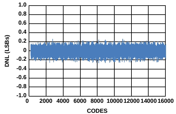
FIGURE 12. DIFFERENTIAL NONLINEARITY
