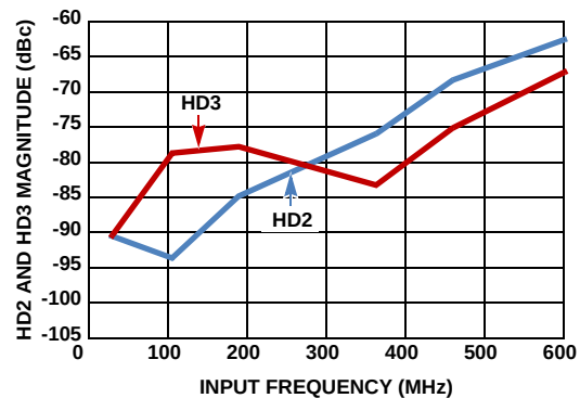
FIGURE 6. HD2 AND HD3 vs f_{IN}
