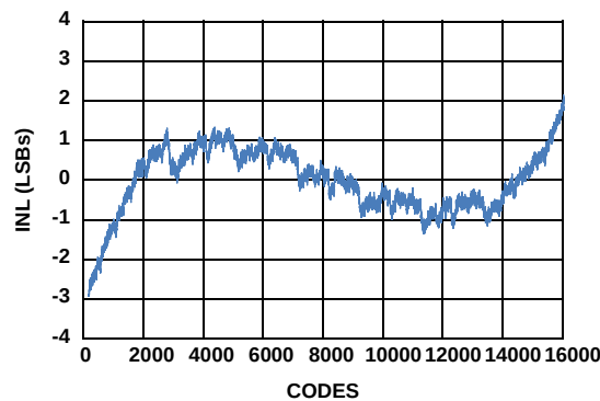
FIGURE 13. INTEGRAL NONLINEARITY
