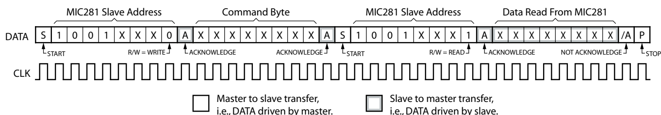
Figure 2. Read_Byte Protocol
