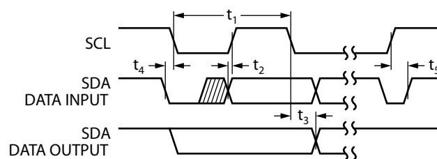
Serial Interface Timing
