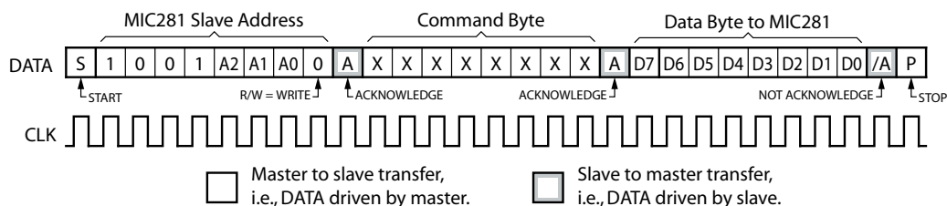
Figure 1. Write_Byte Protocol
