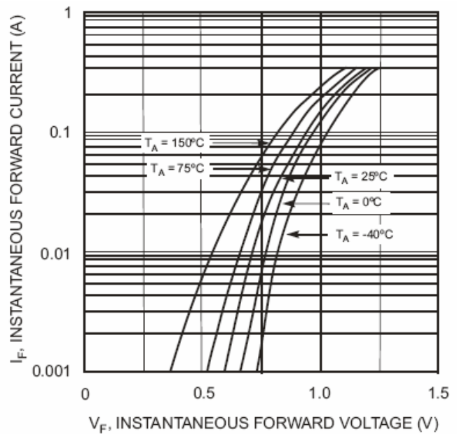
Fig. 2 Forward Characteristics
