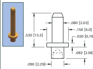
.080 (2.0) PIN - SWAGE MOUNT
