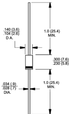
DO-204AC (DO-15)
