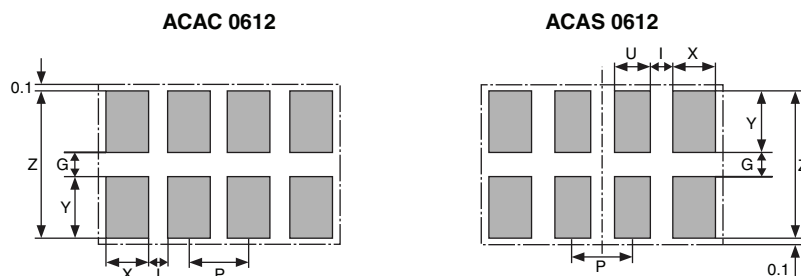
RECOMMENDED SOLDER PAD DIMENSIONS FOR CHIP RESISTOR ARRAYS
