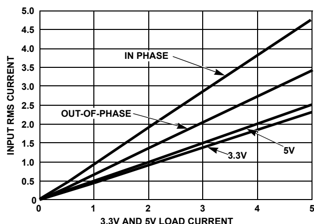
FIGURE 24. INPUT RMS CURRENT vs LOAD
