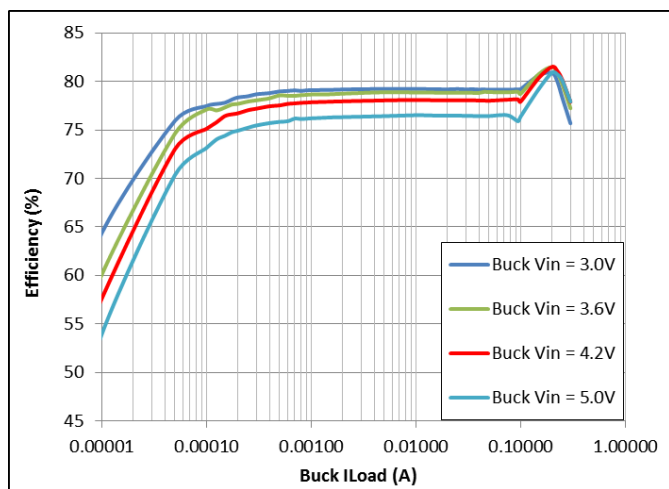
Figure 14: Buck V_{OUT} = 0.6\text{ V}
