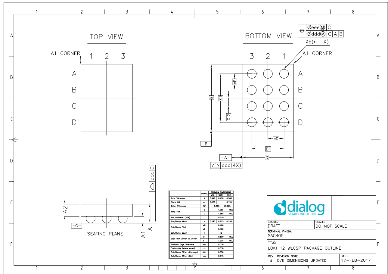
Figure 56: Package Outline Drawing
