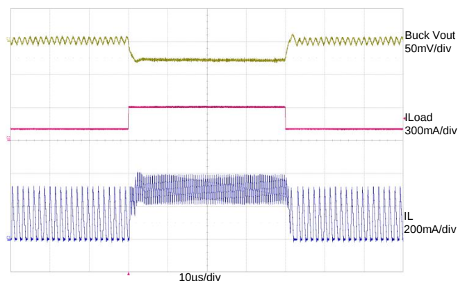
Figure 36: Buck I_{LOAD} = 100 \text{ mA} to 300 \text{ mA} to 100 \text{ mA} ( 0.2 \text{ A}/\mu\text{s} ); Buck V_{IN} = 3.6 \text{ V} , Buck V_{OUT} = 0.9 \text{ V}
