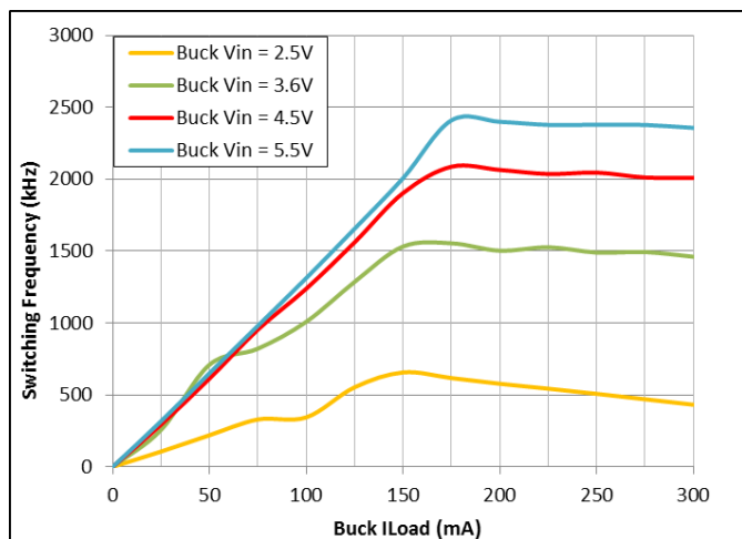
Figure 15: Buck V_{OUT} = 1.9\text{ V}
