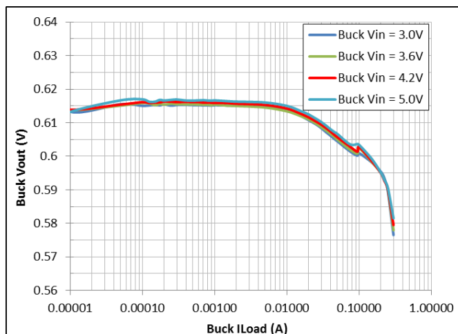
Figure 26: Buck V_{OUT} = 0.6\text{ V}
