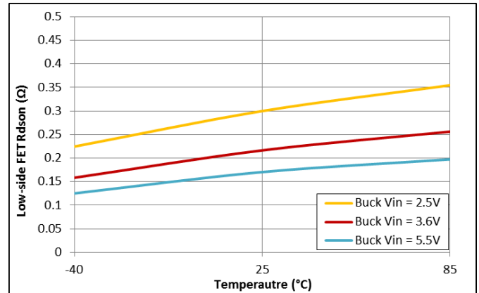
Figure 9: Low-Side FET
