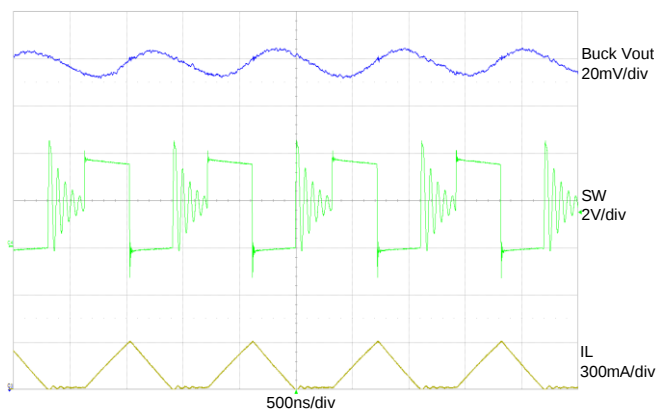
Figure 29: Buck V_{IN} = 3.6\text{ V} , Buck V_{OUT} = 1.8\text{ V} , Buck I_{LOAD} = 100\text{ mA}
