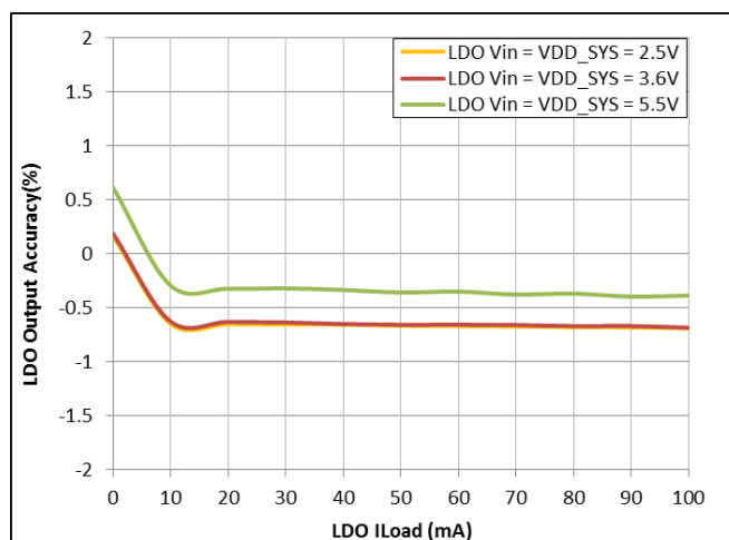
Figure 47: LDO V_{OUT} = 2 \text{ V}
