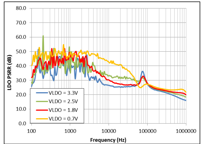
Figure 53: LDO V_{IN} = 3.7 V, LDO I_{LOAD} = 100 mA
