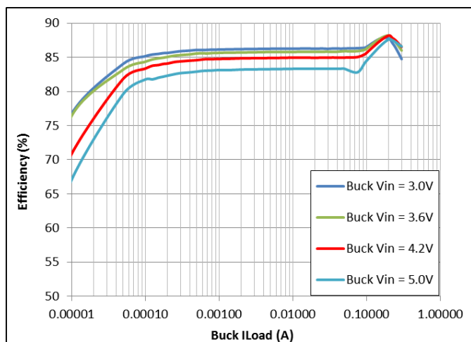
Figure 12: Buck V_{OUT} = 1.2\text{ V}
