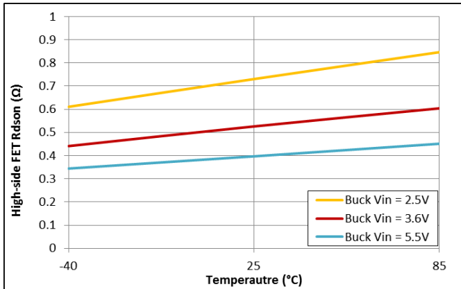
Figure 8: High-Side FET
