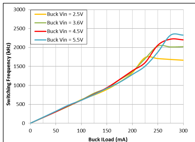
Figure 18: Buck V_{OUT} = 0.6\text{ V}
