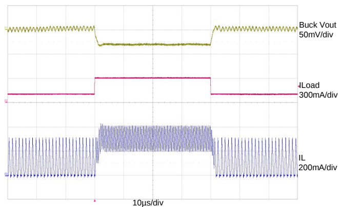
Figure 34: Buck I_{LOAD} = 100 \text{ mA} to 300 \text{ mA} to 100 \text{ mA} ( 0.2 \text{ A}/\mu\text{s} ); Buck V_{IN} = 3.6 \text{ V} , Buck V_{OUT} = 1.2 \text{ V}
