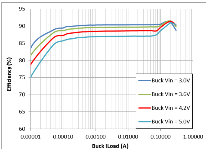
Figure 10: Buck V_{OUT} = 1.9\text{ V}
