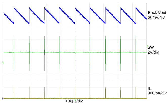
Figure 27: Buck V_{IN} = 3.6\text{ V} , Buck V_{OUT} = 1.8\text{ V} , Buck I_{LOAD} = 1\text{ mA}
