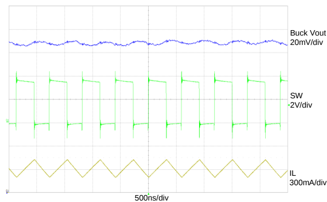
Figure 30: Buck V_{IN} = 3.6\text{ V} , Buck V_{OUT} = 1.8\text{ V} , Buck I_{LOAD} = 300\text{ mA}
