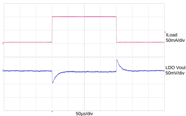
Figure 50: LDO I_{LOAD} = 5 \text{ mA} to 100 \text{ mA} to 5 \text{ mA} (0.1 \text{ A} / 1 \text{ } \mu\text{s}) ; LDO V_{IN} = 3.6 \text{ V} , LDO V_{OUT} = 2 \text{ V}
