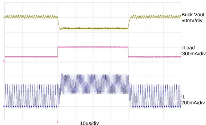
Figure 32: Buck I_{LOAD} = 100 \text{ mA} to 300 \text{ mA} to 100 \text{ mA} ( 0.2 \text{ A}/\mu\text{s} ); Buck V_{IN} = 3.6 \text{ V} , Buck V_{OUT} = 1.8 \text{ V}
