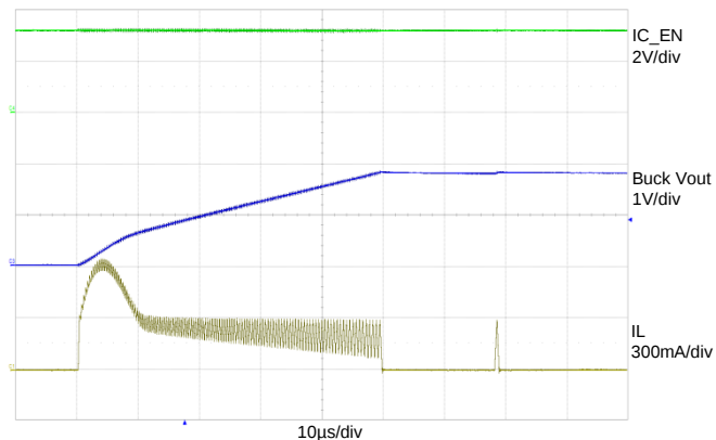
Figure 44: V_{OUT} ramp-up after Enabled (Zoom-in of Figure 43)
