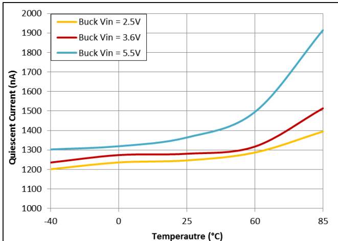
Figure 6: Buck V_{OUT} = 1.8 V , LDO V_{OUT} = 0.8 V
