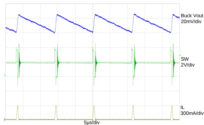
Figure 28: Buck V_{IN} = 3.6\text{ V} , Buck V_{OUT} = 1.8\text{ V} , Buck I_{LOAD} = 10\text{ mA}
