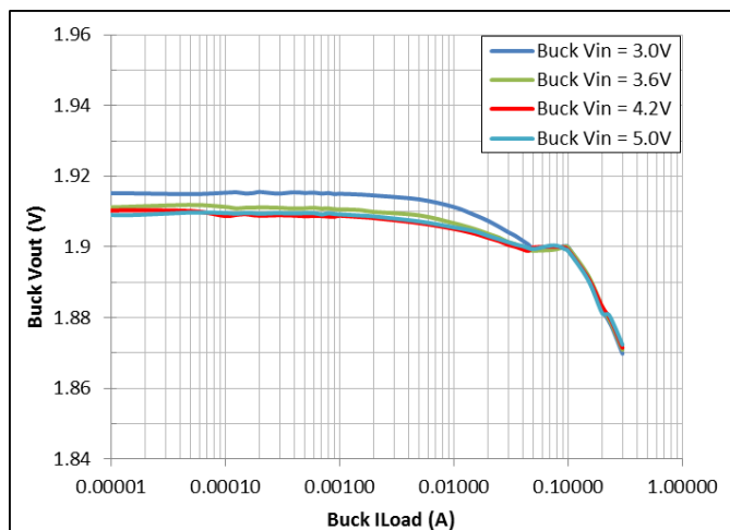
Figure 23: Buck V_{OUT} = 1.9\text{ V}
