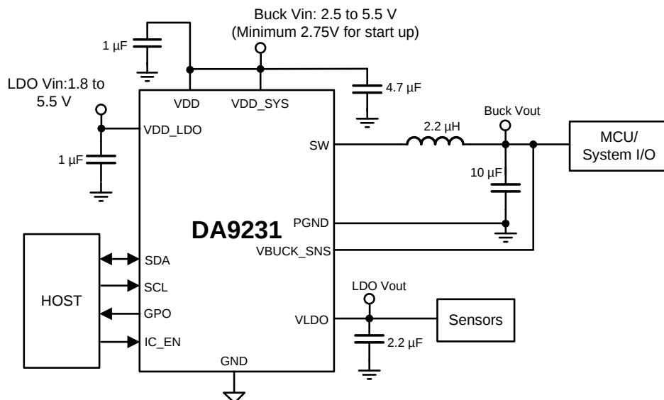
Figure 2: DA9231 Application Diagram
