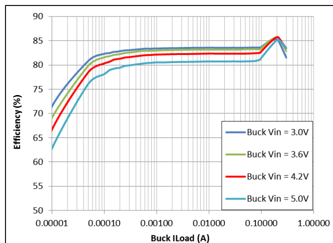
Figure 13: Buck V_{OUT} = 0.9\text{ V}
