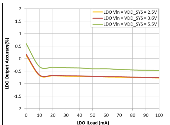
Figure 46: LDO V_{OUT} = 0.8 \text{ V}
