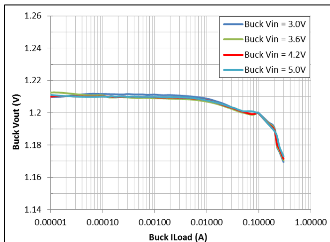
Figure 24: Buck V_{OUT} = 1.2\text{ V}
