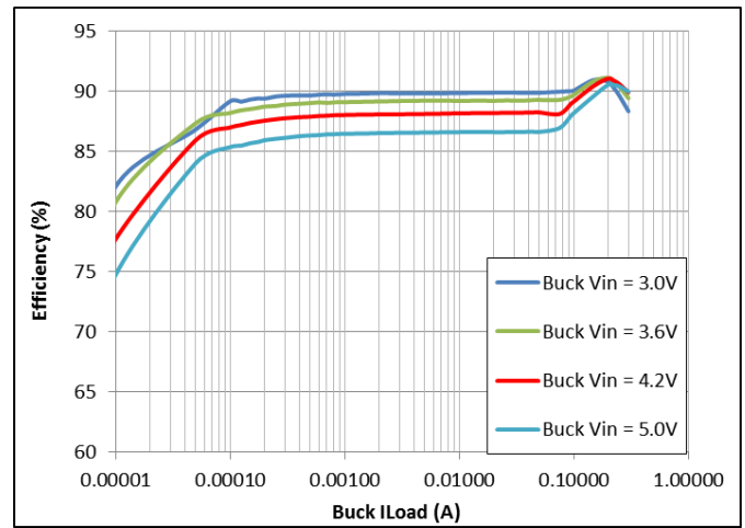
Figure 11: Buck V_{OUT} = 1.8\text{ V}
