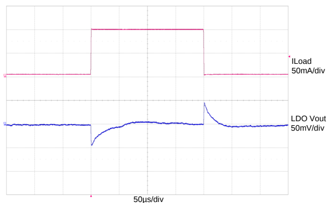
Figure 51: LDO I_{LOAD} = 5 \text{ mA} to 100 \text{ mA} to 5 \text{ mA} (0.1 \text{ A} / 1 \text{ } \mu\text{s}) ; LDO V_{IN} = 3.6 \text{ V} , LDO V_{OUT} = 3.3 \text{ V}
