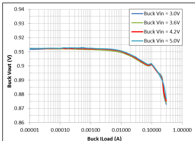
Figure 25: Buck V_{OUT} = 0.9\text{ V}
