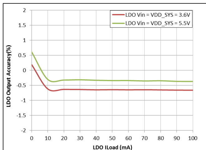
Figure 48: LDO V_{OUT} = 3.3 \text{ V}
