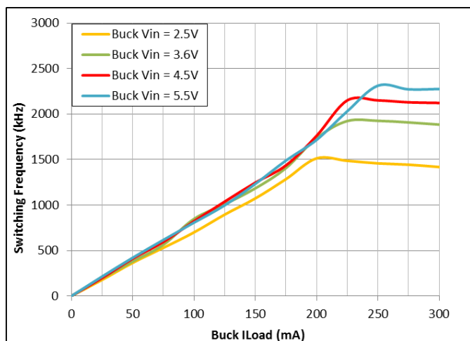
Figure 16: Buck V_{OUT} = 0.9\text{ V}
