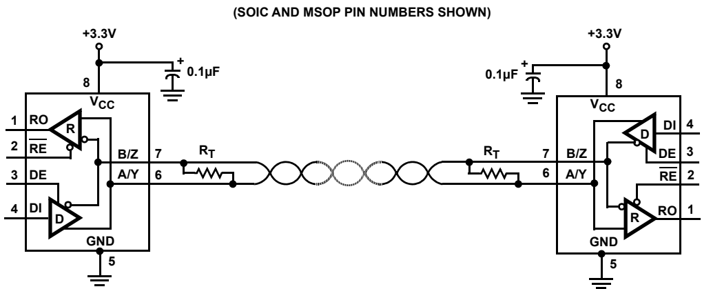
FIGURE 2. ISL3179E
