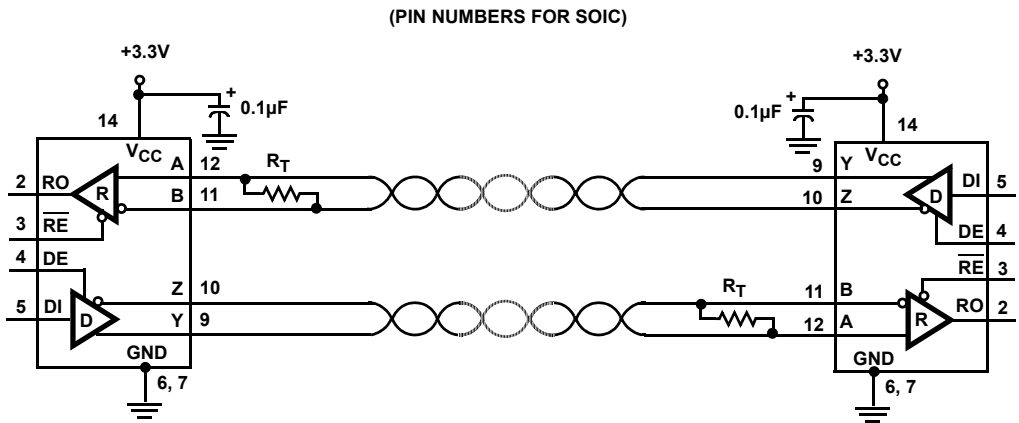
FIGURE 3. ISL3180E
