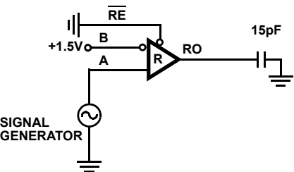
FIGURE 8A. TEST CIRCUIT
