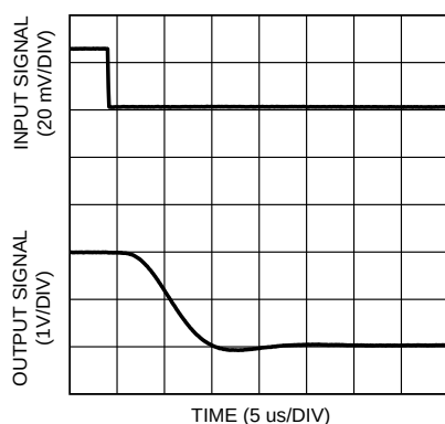
Settling Time (Falling Edge) at V_S = 3.3\text{V} LMP8603
