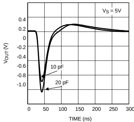
Figure 49. Capacitive Load Response at 5.0V
