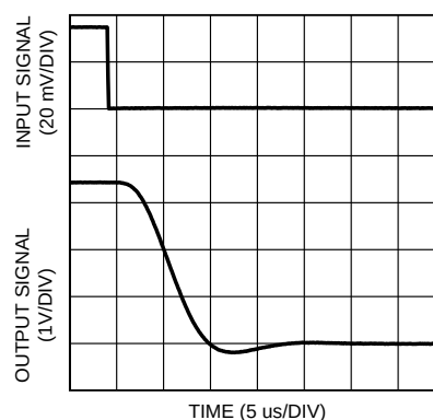
Settling Time (Falling Edge) at V_S = 5\text{V} LMP8603
