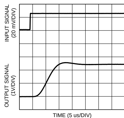
Settling Time (Rising Edge) at V_S = 3.3\text{V} LMP8603
