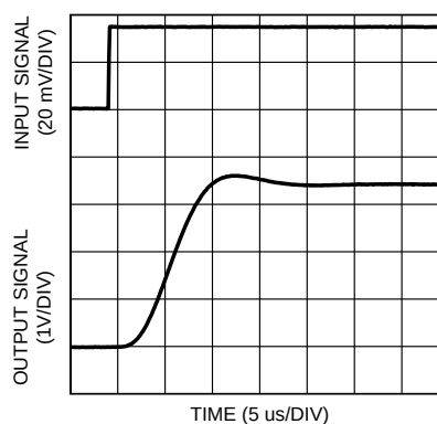
Settling Time (Rising Edge) at V_S = 5\text{V} LMP8603
