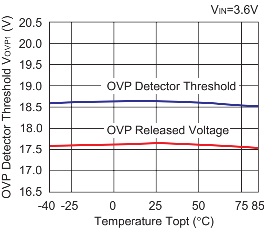
12) OVP Detector Threshold/Released Voltage vs. Temperature R1218x041A
