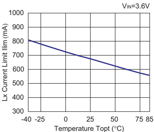
14) Lx Current Limit vs. Temperature R1218x041A
