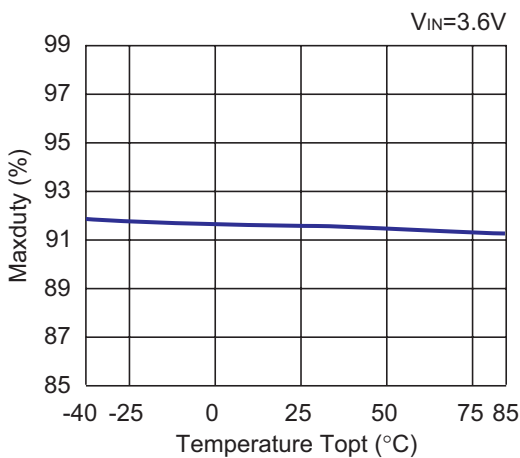
11) Maximum duty cycle vs. Temperature R1218x041A
