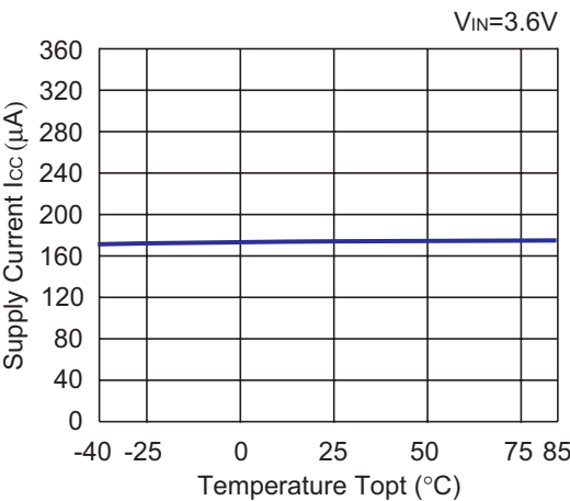
13) Supply Current vs. Temperature R1218x041A
