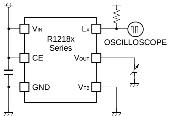
OVP Detector Threshold, OVP Released Voltage Test Circuit
