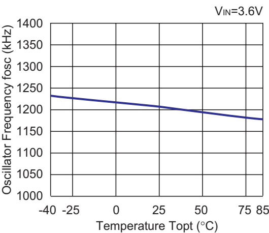
10) Oscillator Frequency vs. Temperature R1218x041A
