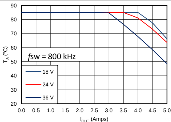
Figure 47. 3.3-V Outputs
