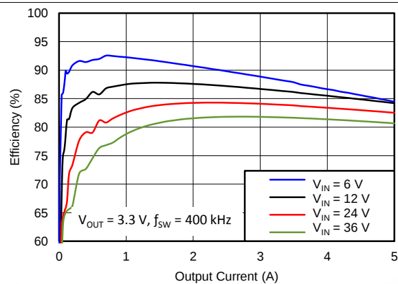
Figure 63. Efficiency vs Load Current
