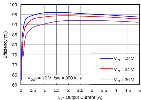
Figure 65. Efficiency vs Load Current
