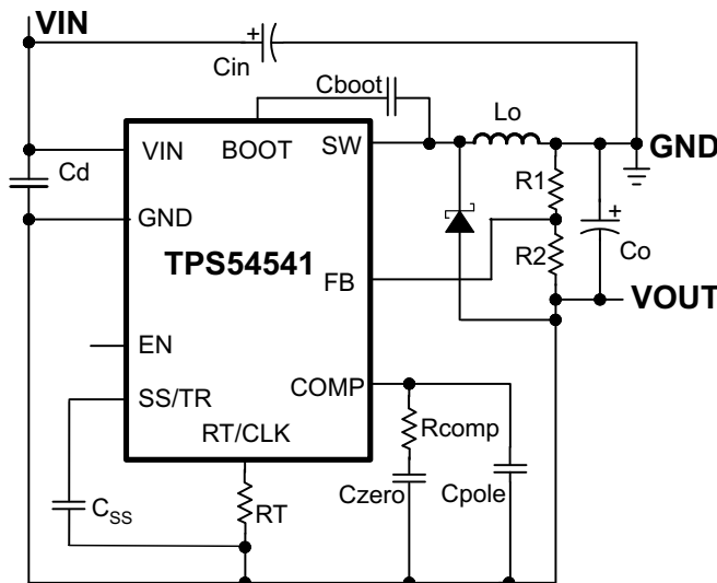
Figure 71. TPS54541 Inverting Power Supply Based on the Application Note, SLVA317
