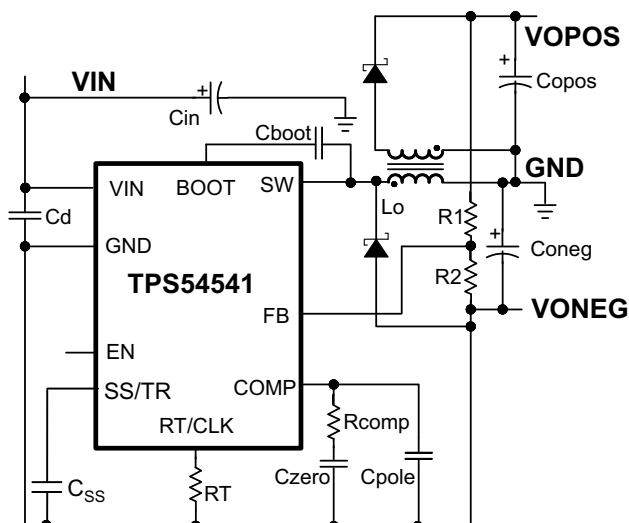
Figure 72. TPS54541 Split Rail Power Supply Based on the Application Note, SLVA369
