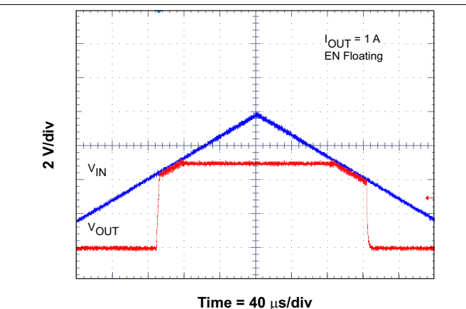
Figure 60. Low Dropout Operation
