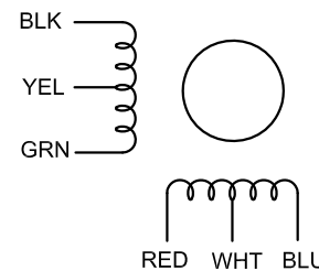
UNIPOLAR
