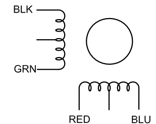
BIPOLAR SERIES
