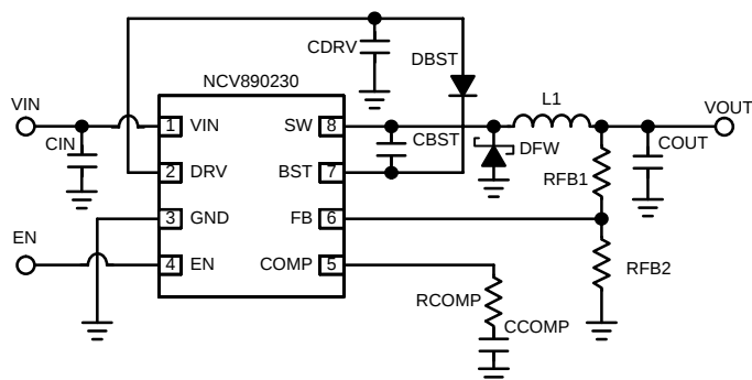
Figure 1. Typical Application
