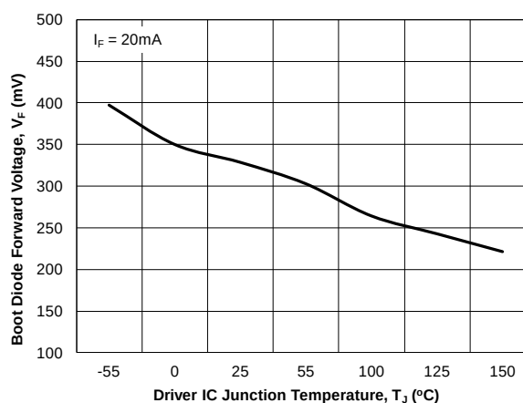
Figure 1.20 Boot Diode Forward Voltage vs. Temperature
