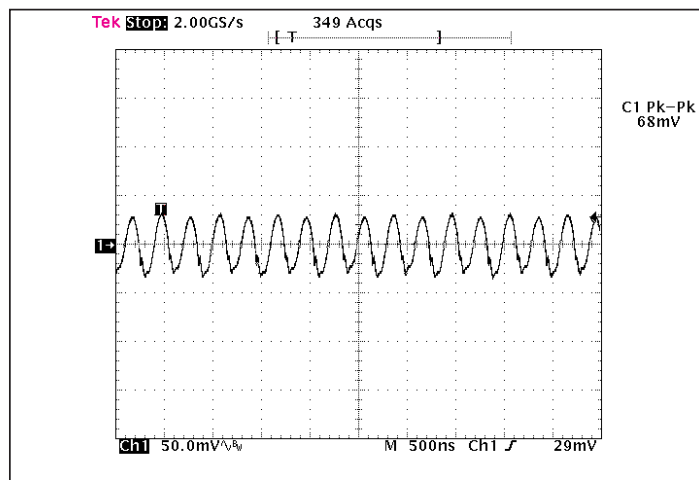
Figure 7 — Output voltage ripple at full load and nominal V_{IN} ; without any external bypass capacitor.
