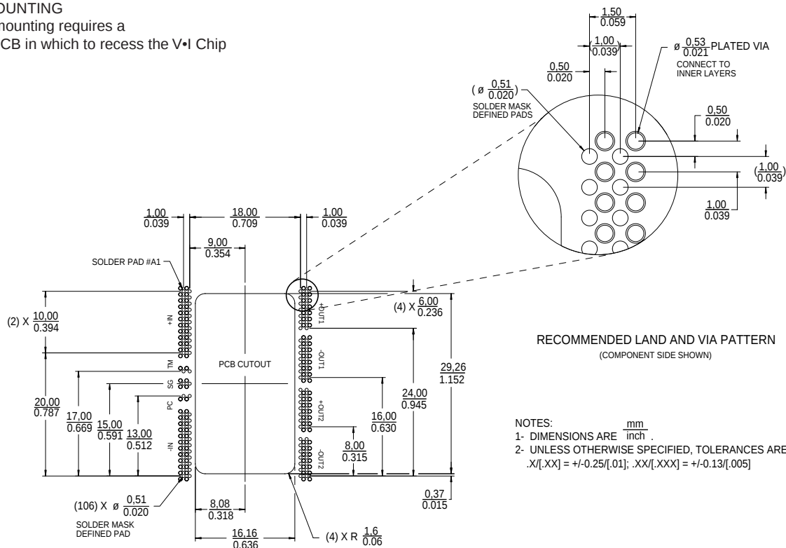
Figure 17—BCM BGA PCB land/VIA layout information; In-board mounting
