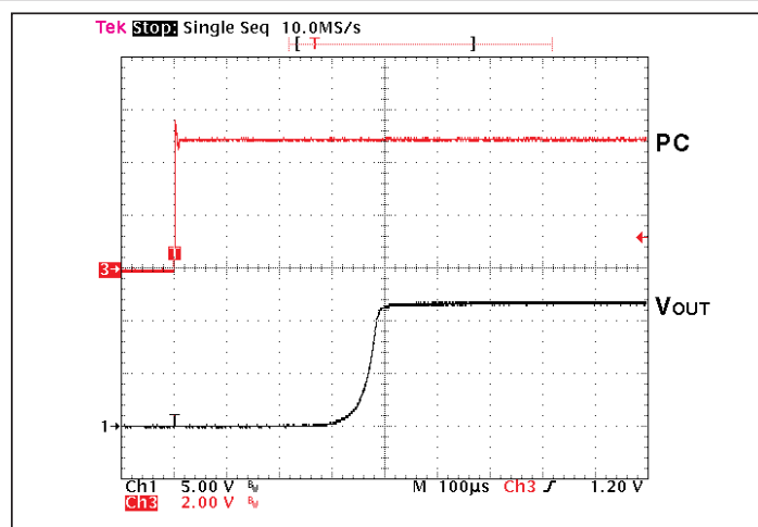
Figure 2 —Output voltage turn-on waveform with PC enabled at full load and nominal V_{IN}
