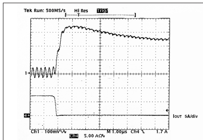
Figure 12 — 8.3-0A transient response with no external bypass capacitance.
