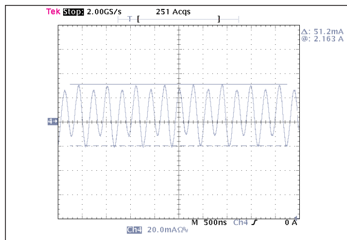
Figure 4 —Input reflected ripple current at full load and nominal V_{IN}
