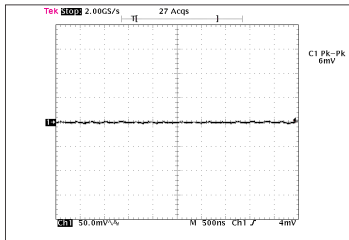
Figure 8 — Output voltage ripple at full load and nominal V_{IN} with 1\ \mu\text{F} ceramic external bypass capacitor.
