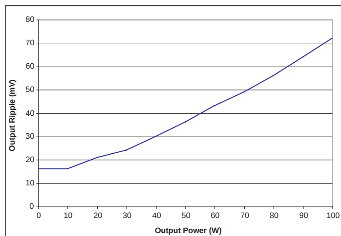
Figure 10 — Output voltage ripple vs. output power at nominal line without any external bypass capacitor.
