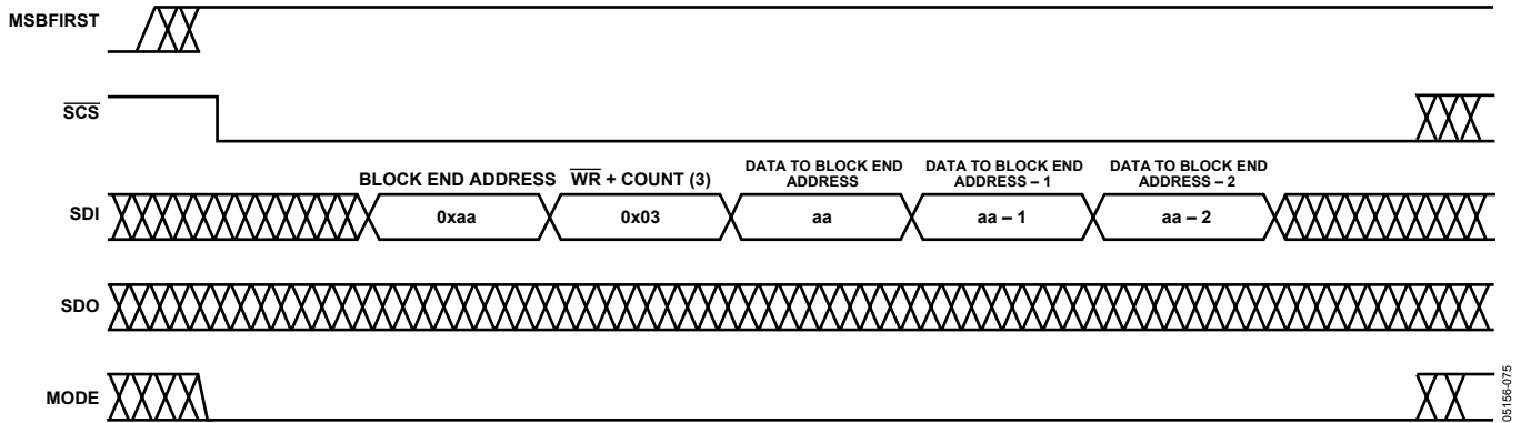
Figure 61. Serial Write of Three Bytes with MSBFIRST = 1 (All Words are Written MSB first)
