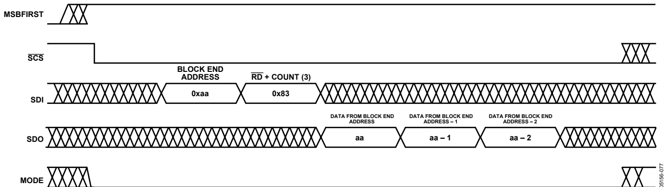
Figure 63. Serial Read of Three Bytes with MSBFIRST = 1 (All Words are Written or Read MSB First)
