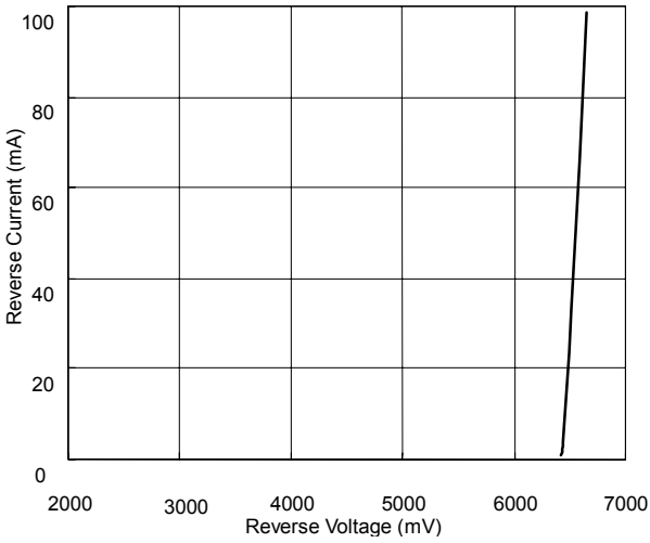
ZD5234B Reverse Current vs Reverse Voltage
