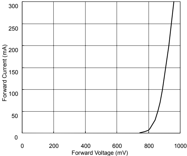
ZD5229B Forward Current vs Forward Voltage
