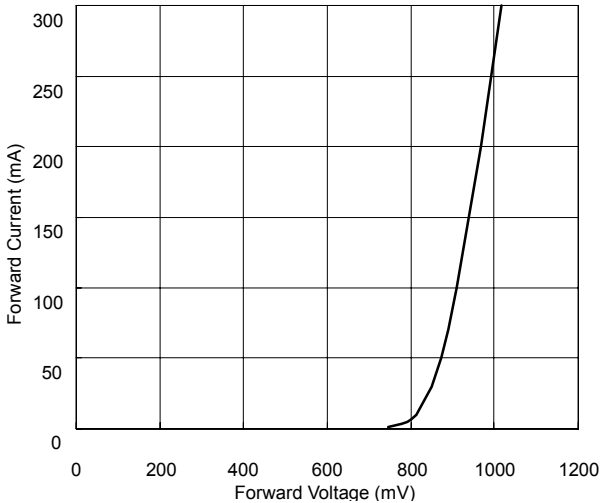
ZD5243B Forward Current vs Forward Voltage
