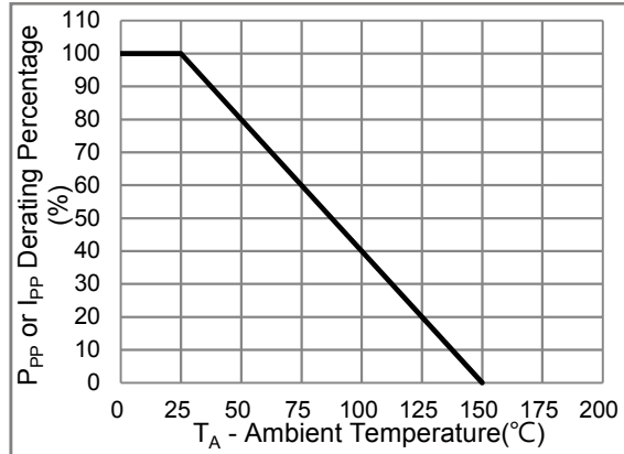
Fig.2 Derating Curve
