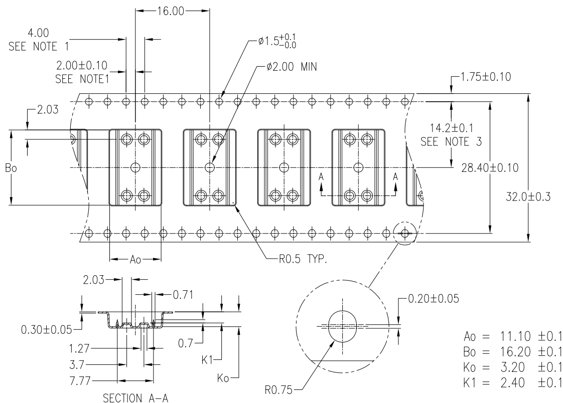
Figure 15. 48-Pin SSOP Carrier Tape Drawing
